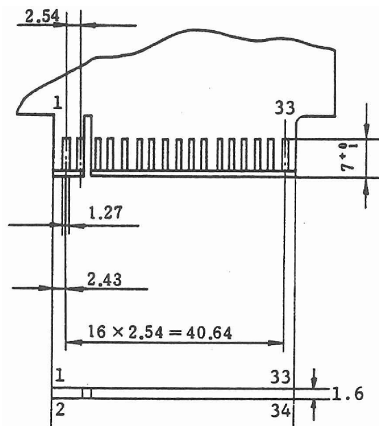
Fig. 2-1 Signal connector
