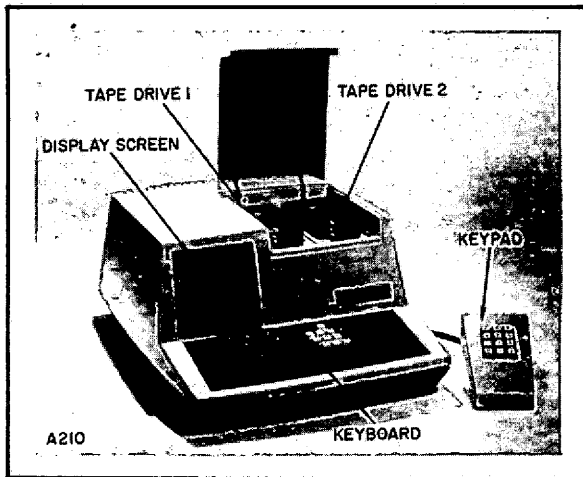
Fig. 1-1. Model 1501 Intelligent Terminal
