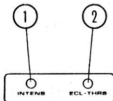
Abb. 3-8: Trimpotentiometer
