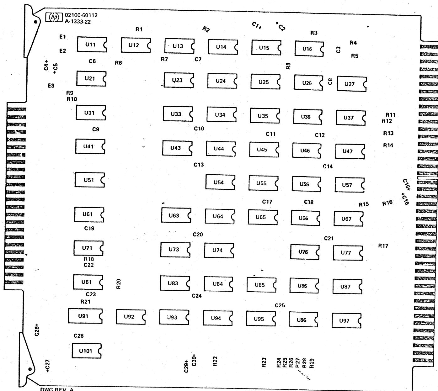
Figure 2-5. A4 Microinstruction Decoder 2 Card, Parts Location Diagram
