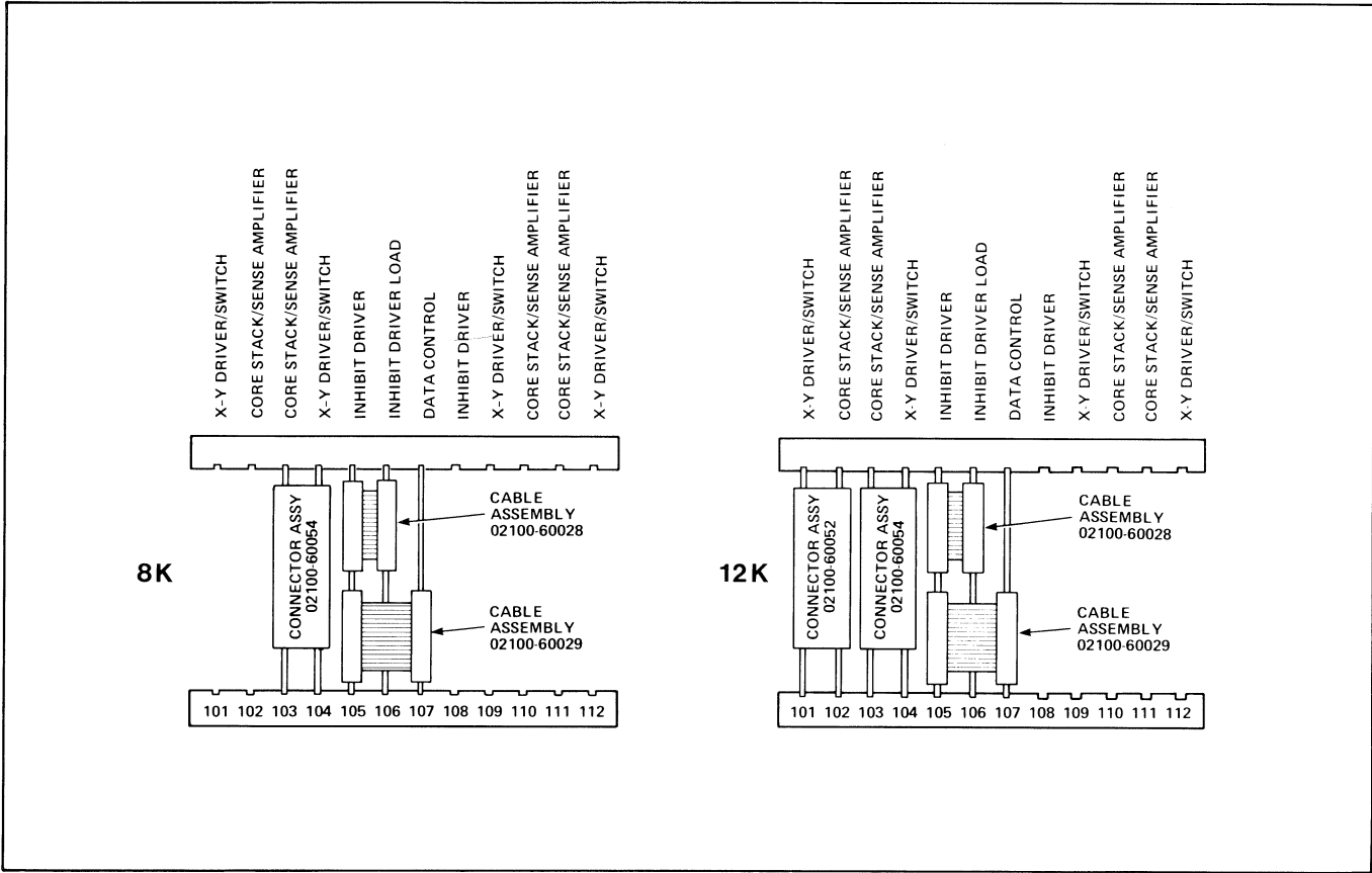
Figure 1. Card Cage Loading Configuration for 8K and 12K Memory Size
