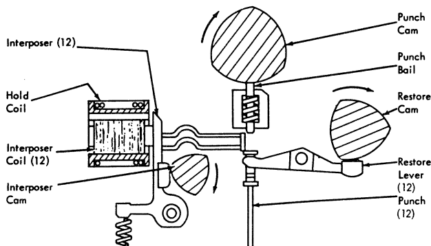
Figure 2-16. Punch Unit Operation
