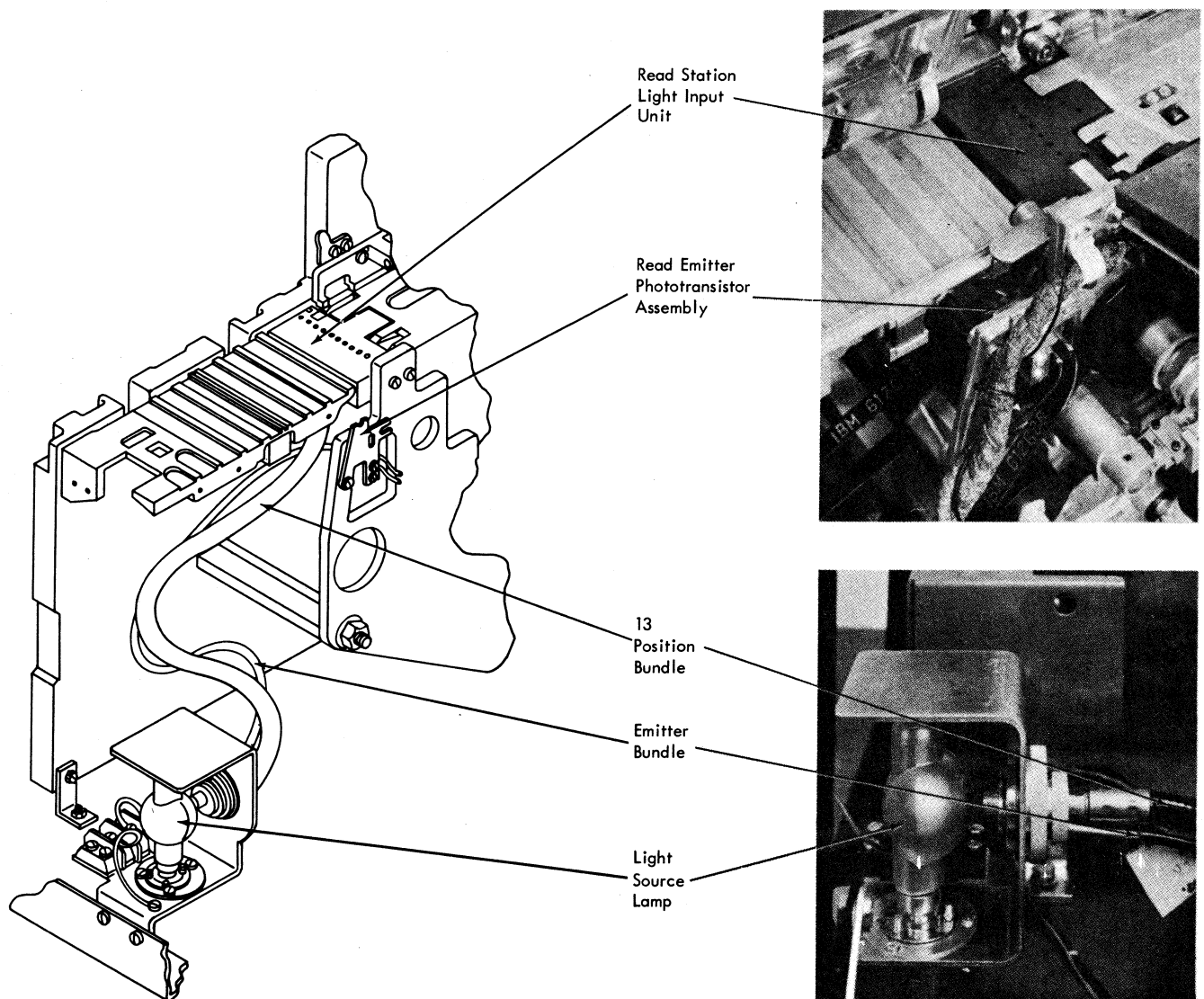
Figure 2-15. Light Source
