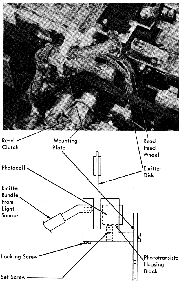
Figure 2-25. Read Emitter
