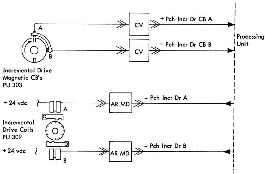
Figure 3-11. 1442 Model 5 Incremental Drive Signals
