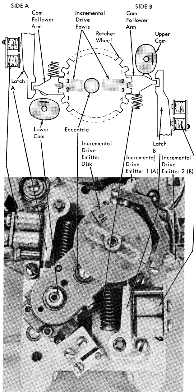
Figure 2-19. Incremental Drive Unit
