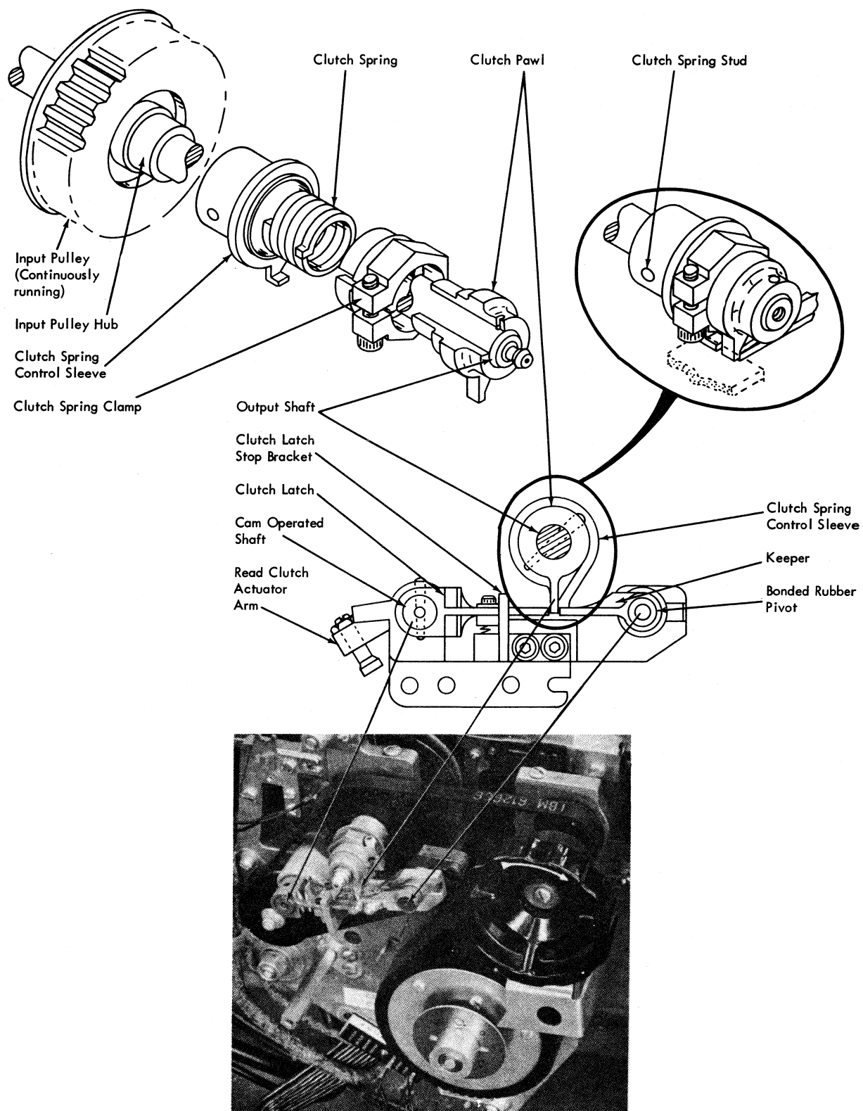
Figure 2-6. Read Clutch
