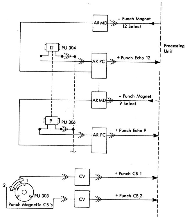
Figure 3-8. 1442 Model 5 Punching Circuits
