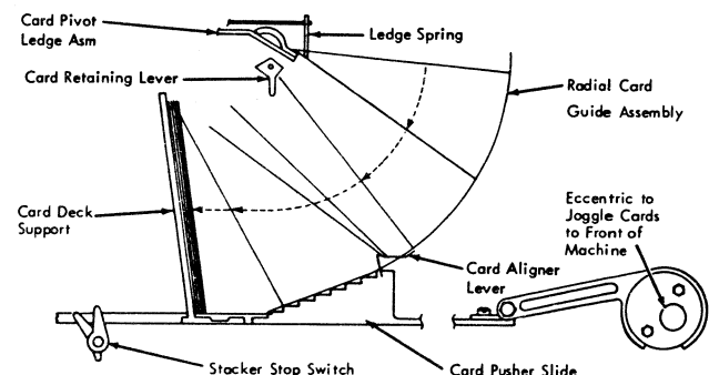
Figure 2-12. Stacker Operation
