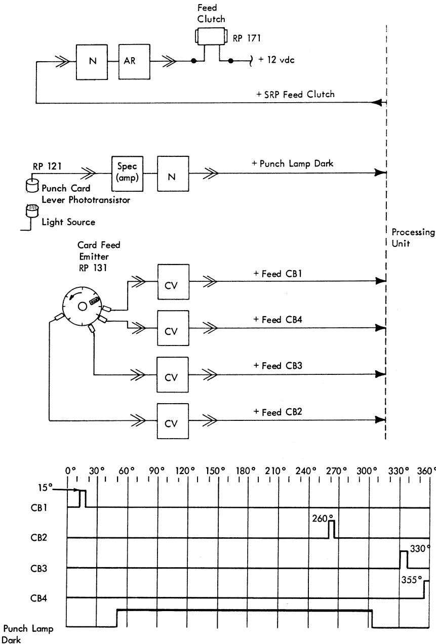
Figure 3-6. 1442 Models 6 and 7 Card Feed Signals
