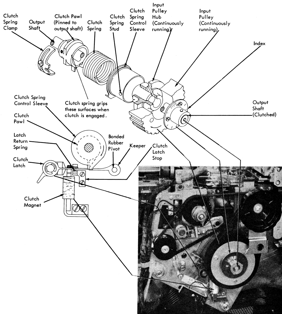
Figure 2-5. Card Feed Clutch
