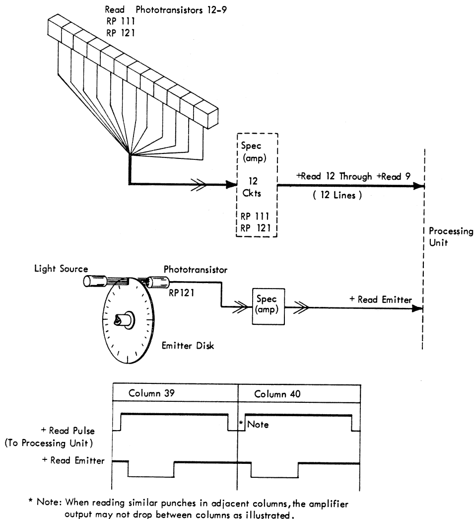
Figure 3-7. 1442 Models 6 and 7 Card Read Signals
