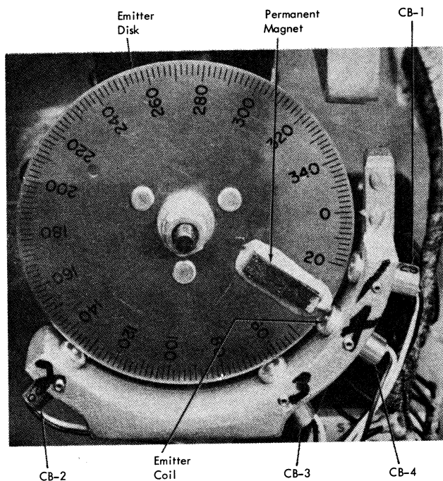
Figure 2-23. Card Feed Emitter
