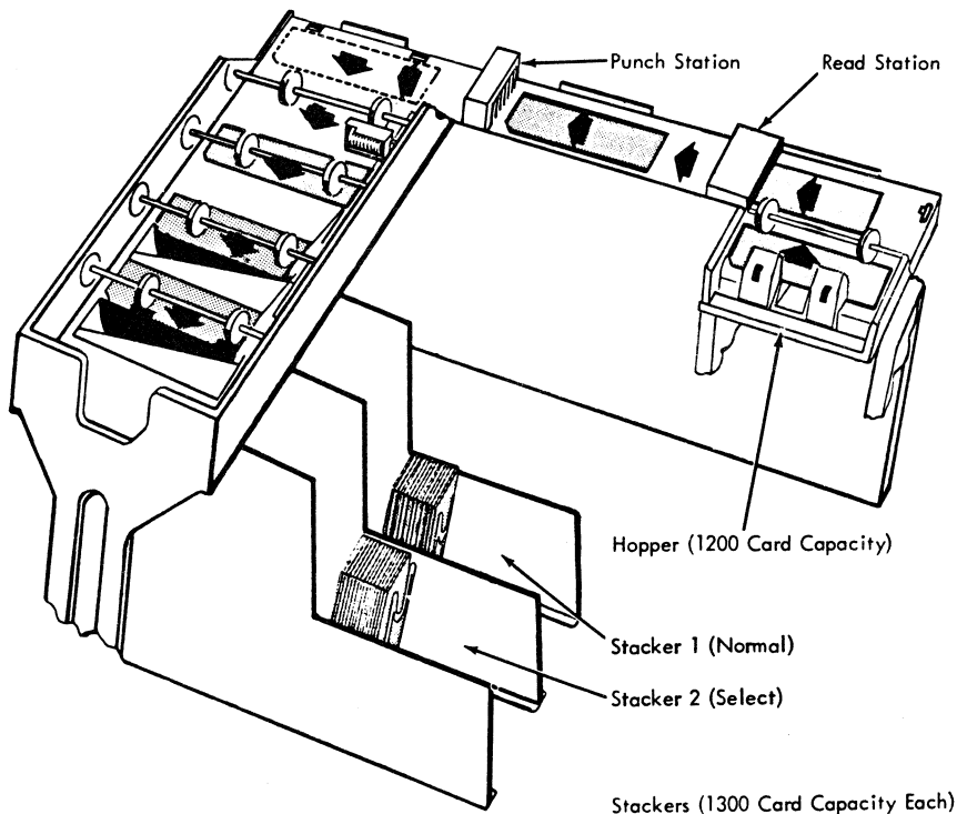
Figure 1-1. Card Path
