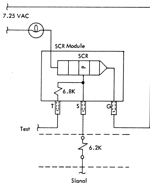
Figure 5-6. OR-ID Circuit
