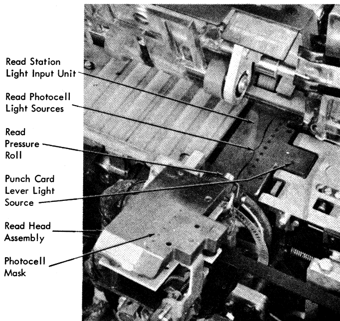
Read Station Open
