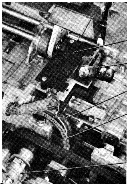
Read Station Closed
