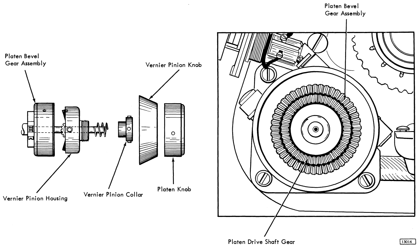
Figure 2-17. Platen Vernier
