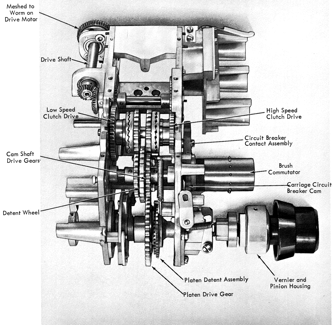
Figure 2-13. Carriage Drive Unit (Removed from Carriage)
