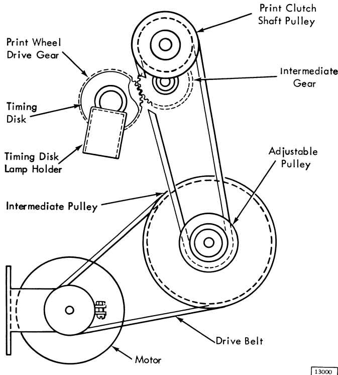
Figure 2-1. Motor and Drive (Left end view)
