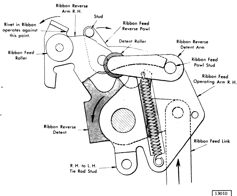
Figure 2-11. Ribbon Reversing Mechanism
