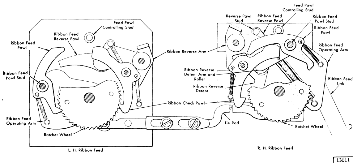
Figure 2-12. Ribbon Feed Mechanism (Feeding to Left)
