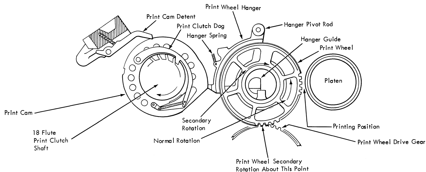
Figure 2-4. Print Cam Mechanism
