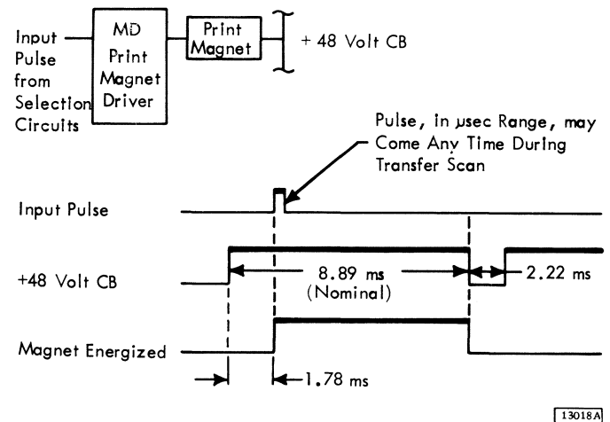
Figure 3-2. Print Magnet Driver Operation
