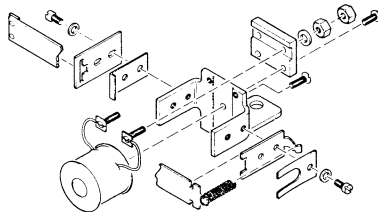
PRINT SUPPRESSION AND MASTER CARD INSERTION MAGNET ASSEMBLY FIGURE 48
