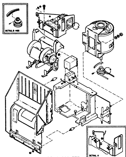
CARD TRANSPORT ASMS FOR STD, STD/HSS, STD/IGP AND SC FEATURES FIGURE 13, SHEET 1 OF 7
