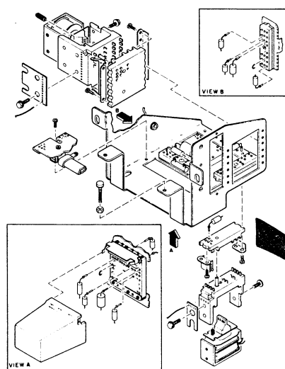
STACKER MOUNTING BRACKET AND TERMINAL BLOCK ASSEMBLY FIGURE 39
