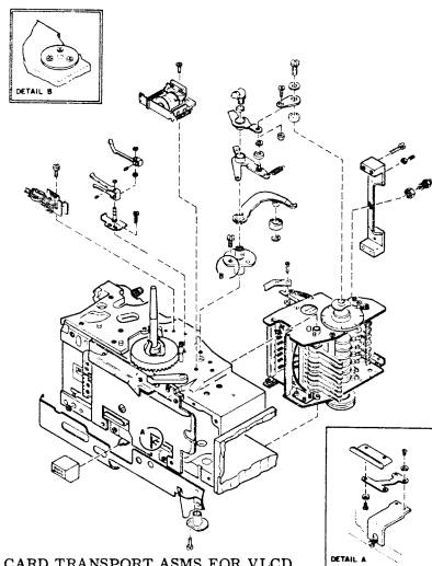
CARD TRANSPORT ASMS FOR VLCD, VLCD/HSS AND SELF CHECK FEATURE FIGURE 14, SHEET 3 OF 7
