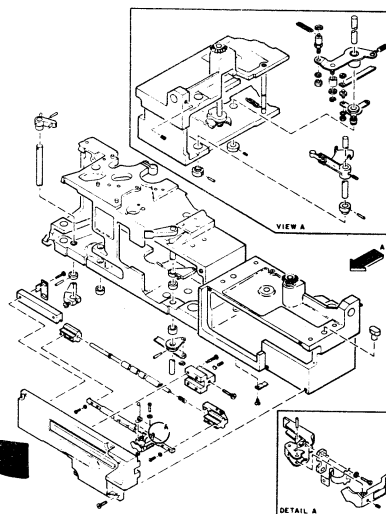
CARD TRANSPORT ASMS FOR VLCD, VLCD/HSS AND SELF CHECK FEATURES FIGURE 14, SHEET 7 OF 7
