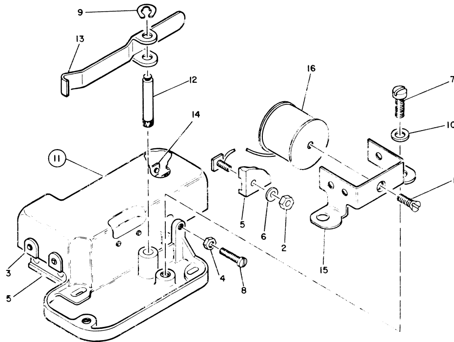
FIGURE 41. LATCH MAGNET ASSEMBLY. SEE LIST 41.
