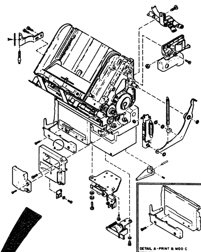
CARD TRANSPORT ASMS FOR STD, STD/HSS, STD/IGP AND SC FEATURES FIGURE 13, SHEET 6 OF 7
