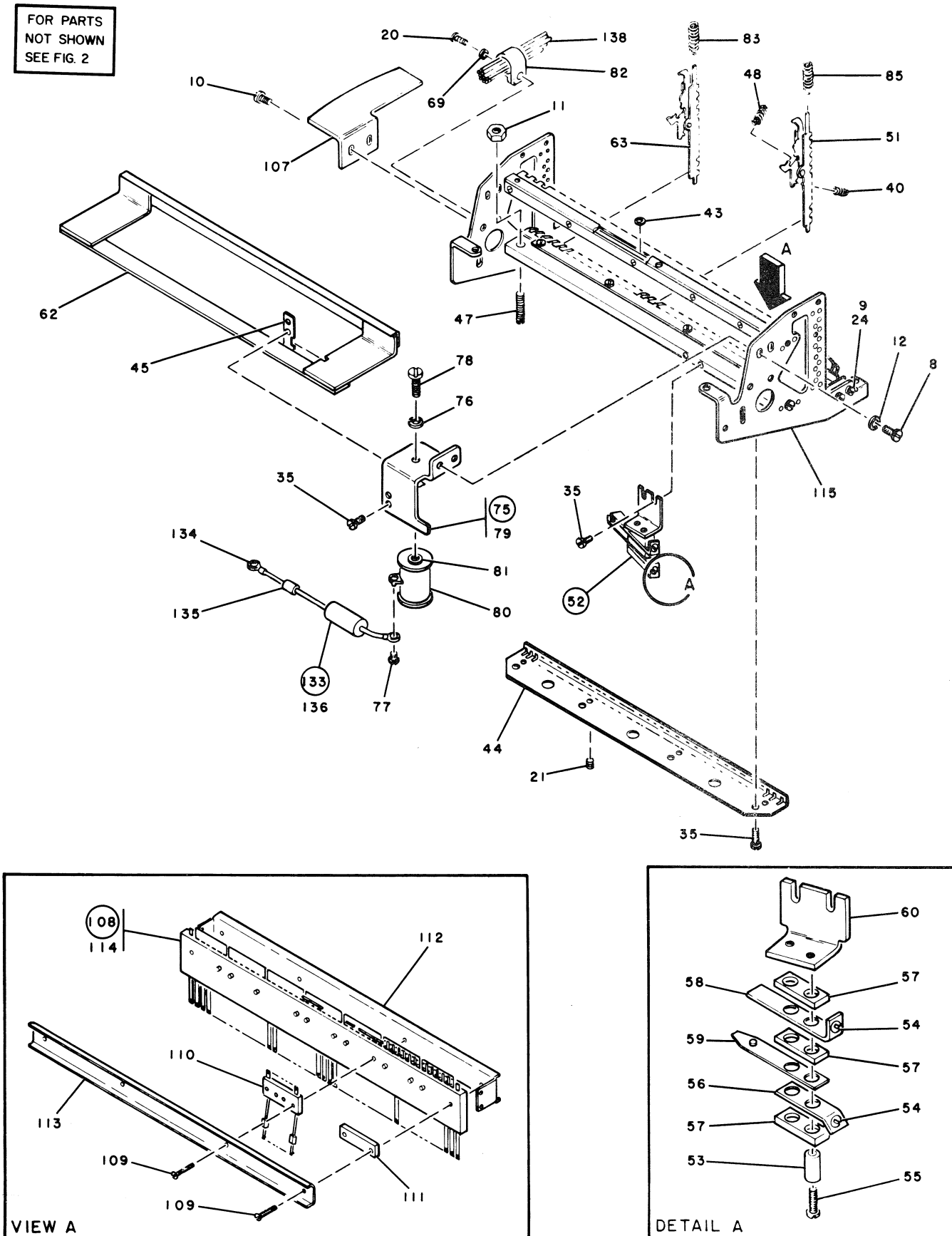
FIGURE 5. COMBINATION KEYBOARDS AND COVER ASSEMBLIES. SHEET 3 OF 5. SEE LIST 5.
