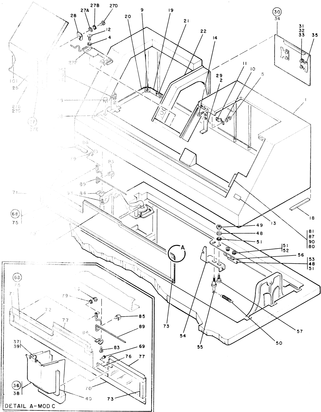
FIGURE 1. STANDARD AND FEATURE COVER ASSEMBLIES. SHEET 2 OF 2.
