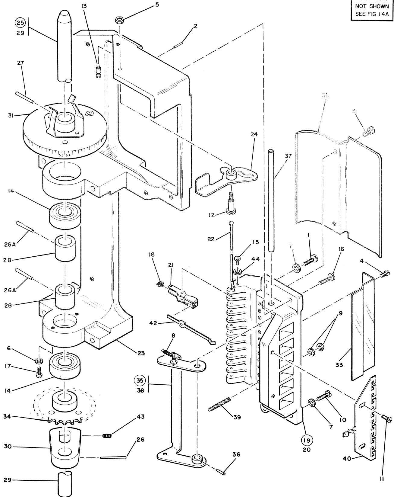
FIGURE 37. AUXILIARY UNIT SENSING ASSEMBLY. SEE LIST 37.
