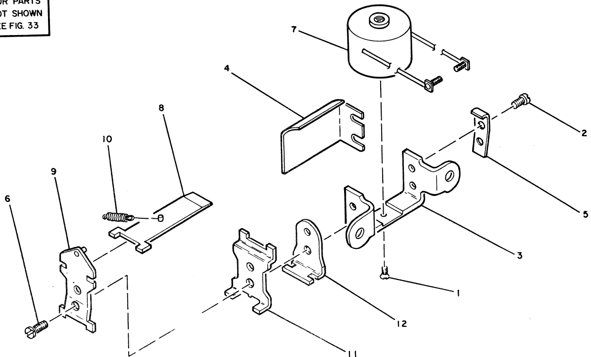
FIGURE 35. PUNCH CLUTCH MAGNET ASSEMBLY. SEE LIST 35.
