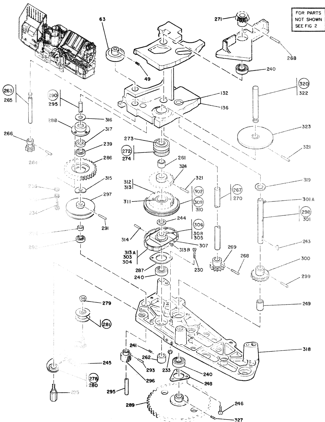
FIGURE 13. CARD TRANSPORT ASMS FOR STD, STD/HSS, STD/IGP AND S.C. FEATURES. SHEET 5 OF 7. SEE LIST 13.
