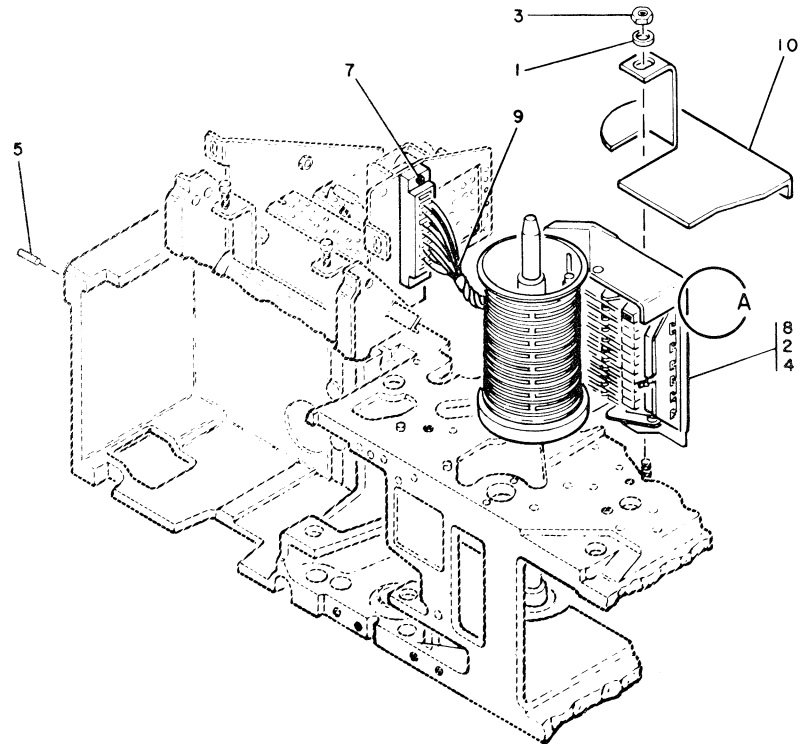
FIGURE 14A. AUXILIARY DUPLICATION AND HIGH SPEED SKIP BACK FRAME MOUNTING. SEE LIST 14A.
