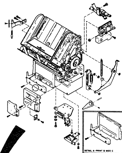
CARD TRANSPORT ASMS FOR STD, STD/HSS, STD/IGP AND SC FEATURES FIGURE 13, SHEET 6 OF 7
