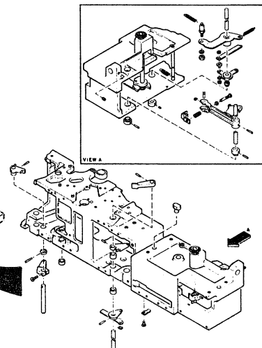
CARD TRANSPORT ASMS FOR STD, STD/HSS, STD/IGP AND SC FEATURES FIGURE 13, SHEET 7 OF 7
