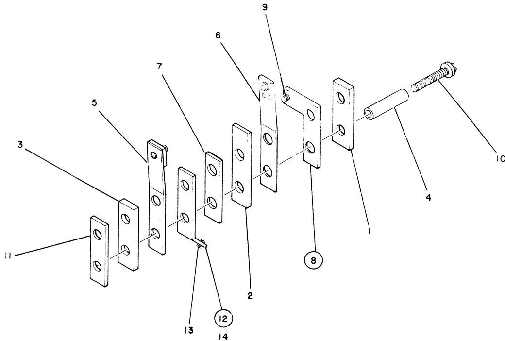
FIGURE 8. DUPLICATION AND ALPHA CONTACT ASSEMBLY. SEE LIST 8.
