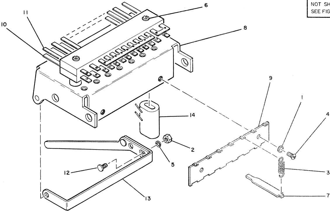
FIGURE 34. PUNCH MAGNET ASSEMBLY. SEE LIST 34.
