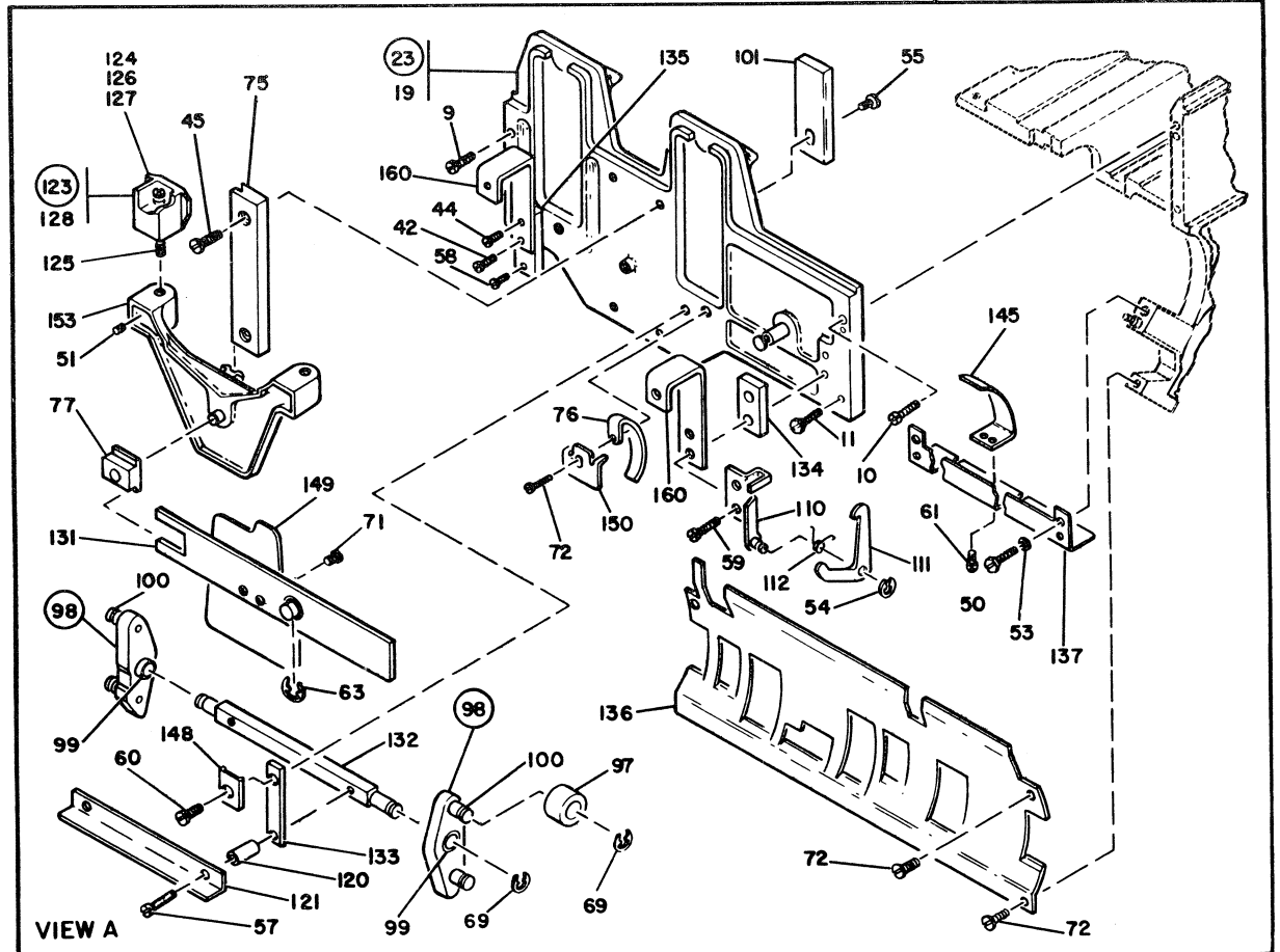
FIGURE 16. VARIABLE LENGTH CARD FEED ASSEMBLIES. SHEET 2 OF 2. SEE LIST 16.
