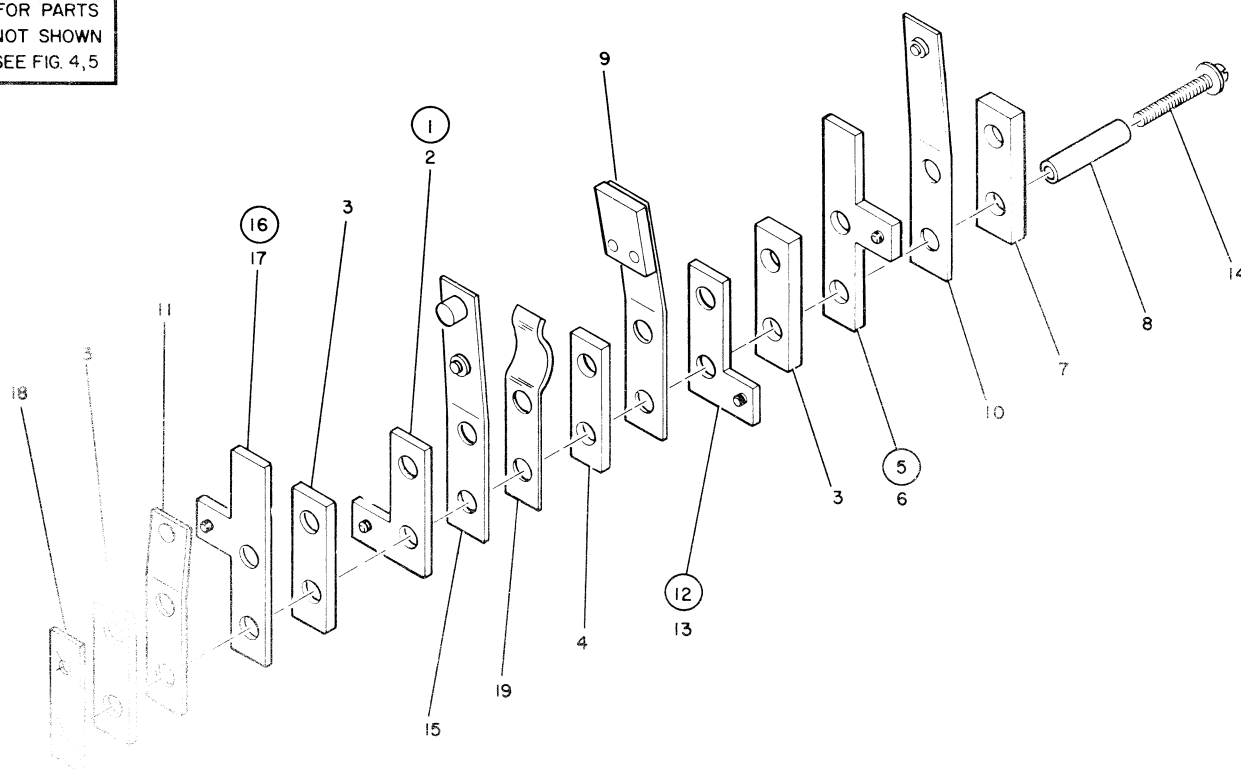
FIGURE 9. MULTI-PUNCH CONTACT ASSEMBLY. SEE LIST 9.
