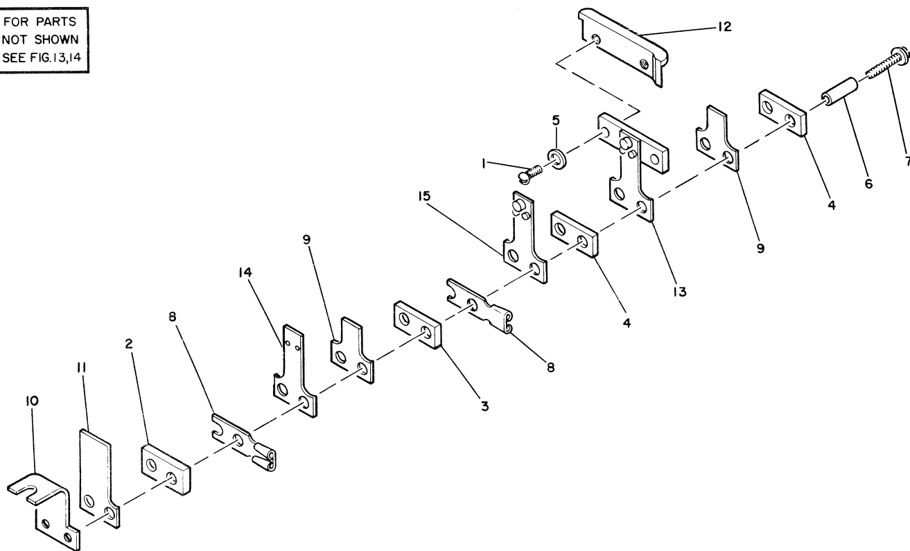
FIGURE 47. DETAIL STATION CARD LEVER ASSEMBLY. SEE LIST 47.
