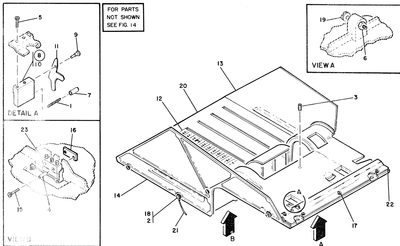
FIGURE 19. VLCD STACKER BED PLATE ASSEMBLY. SEE LIST 19.
