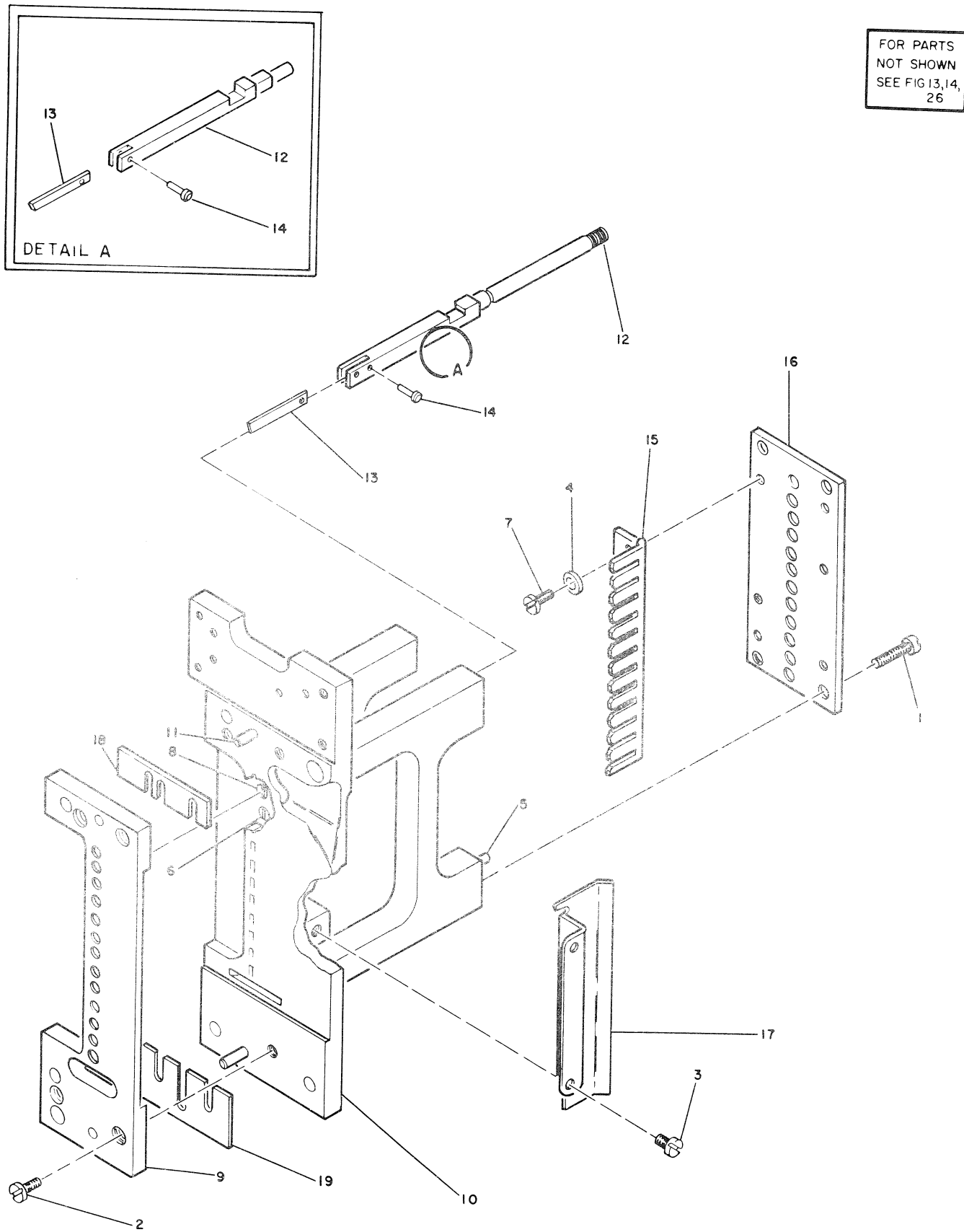
FIGURE 26. DIE AND PUNCH GUIDE ASSEMBLIES. SEE LIST 26
