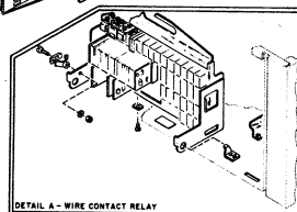
29 CARD PUNCH FINAL ASSEMBLY FIGURE 2, SHEET 3 OF 3
