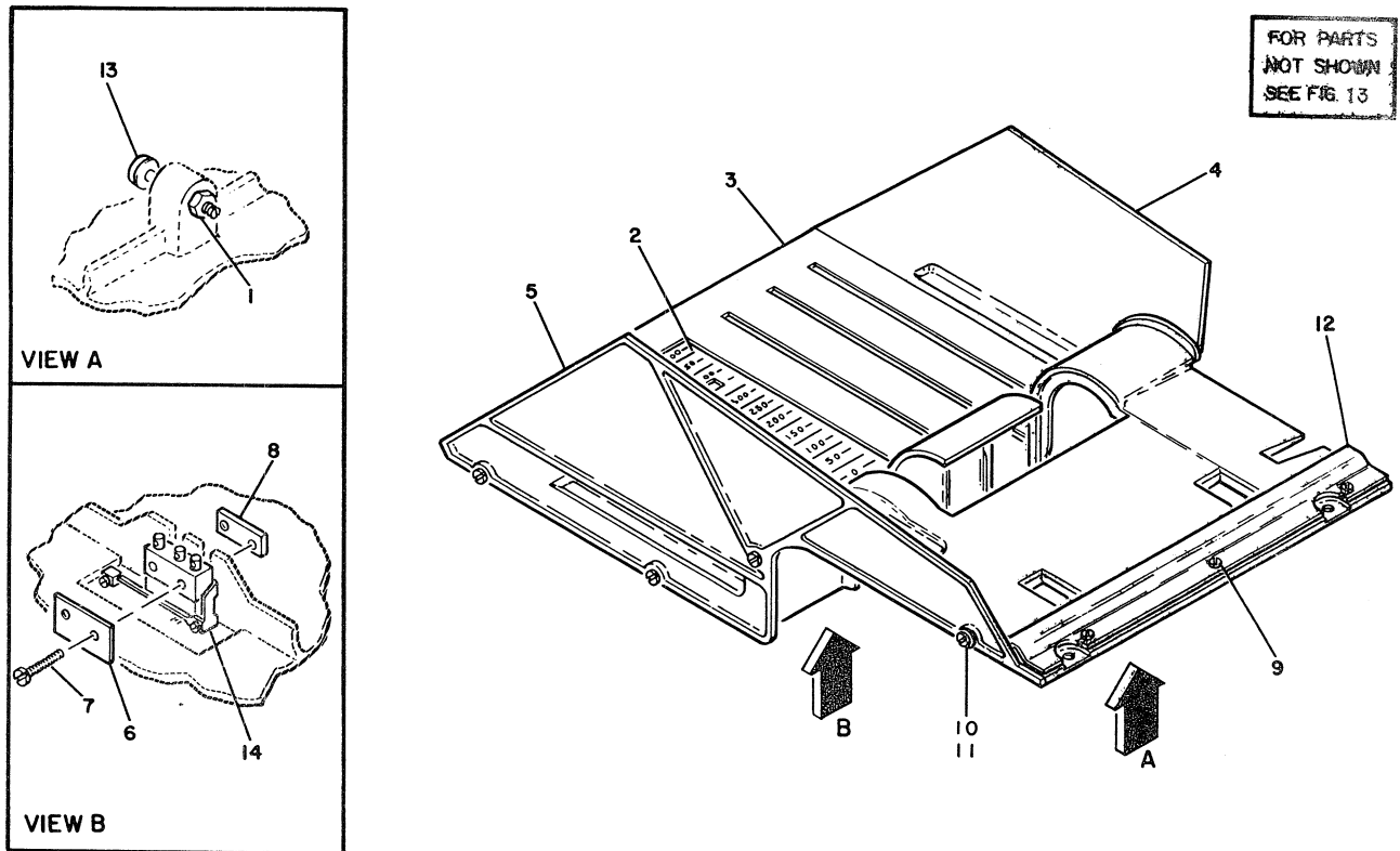
FIGURE 18. STACKER BED PLATE ASSEMBLY. SEE LIST 18.
