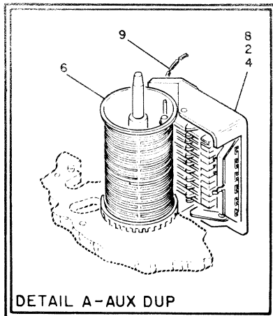
FIGURE 14A. AUXILIARY DUPLICATION AND HIGH SPEED SKIP BACK FRAME MOUNTING. SEE LIST 14A.
