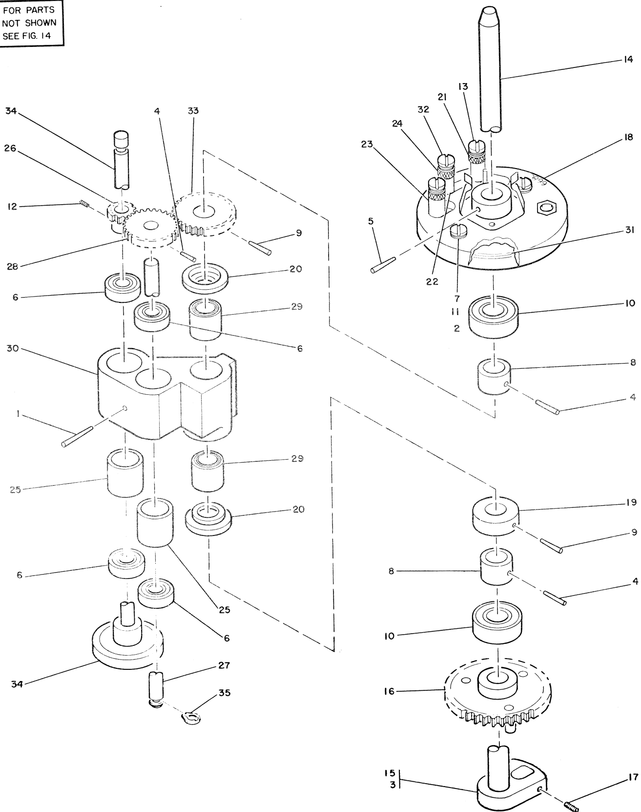
FIGURE 31. VLCD PROGRAM DRUM SHAFT ASSEMBLY. SEE LIST 31.
