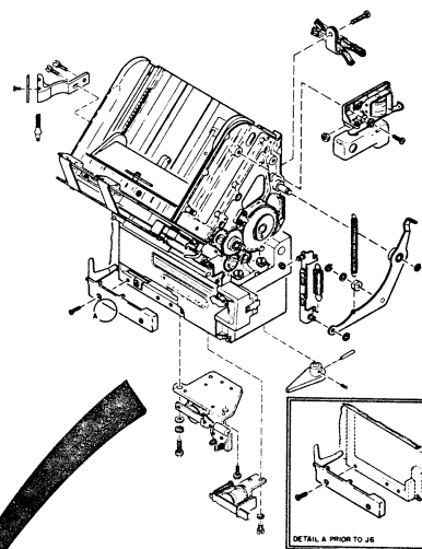
CARD TRANSPORT ASMS FOR VLCD, VLCD/HSS AND SELF CHECK FEATURES FIGURE 14, SHEET 6 OF 7
