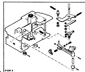
CARD TRANSPORT ASMS FOR STD, STD/HSS, STD/IGP AND SC FEATURES FIGURE 13, SHEET 6 OF 7
