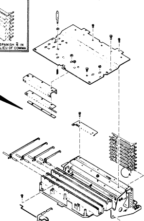
COMBINATION KEYBOARDS AND COVER ASSEMBLIES FIGURE 5, SHEET 1 OF 5
