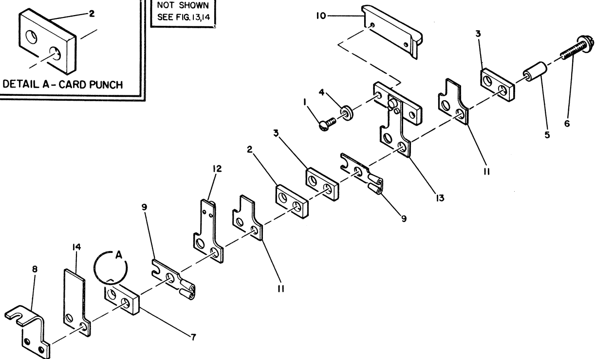
FIGURE 43. CARD PUNCH AND CARD READ LEVER ASSEMBLIES. SEE LIST 43.
