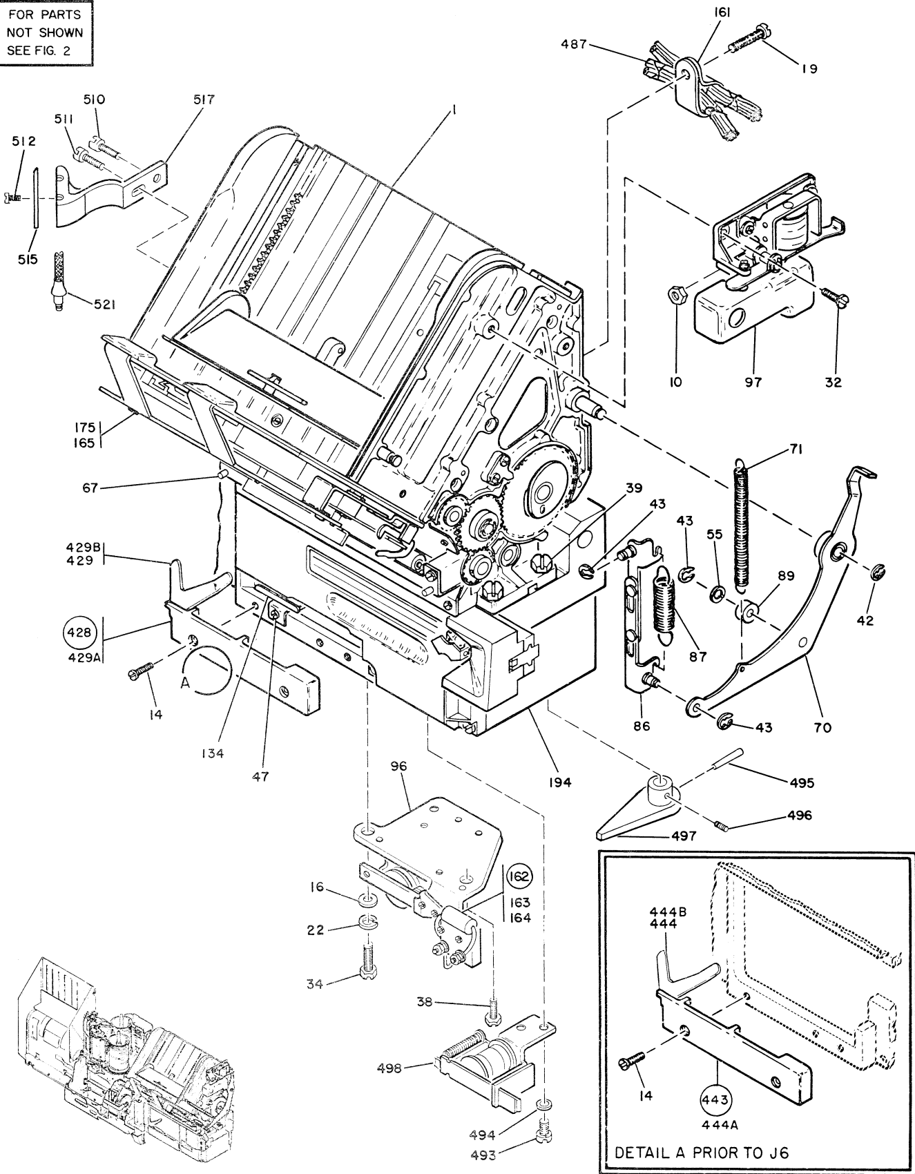
FIGURE 14. CARD TRANSPORT ASSEMBLIES FOR VLCD, VLCD/HSS AND SELF CHECK FEATURE. SHEET 6 OF 7. SEE LIST 14.
