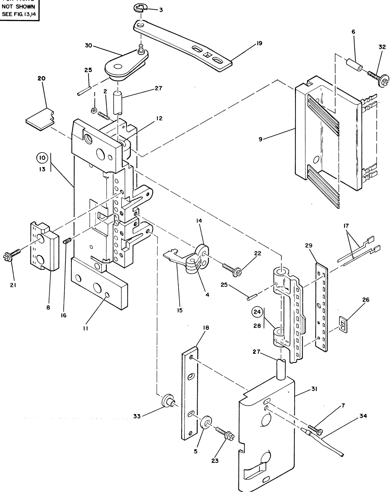
FIGURE 46. PIN SENSING UNIT ASSEMBLIES. SEE LIST 46.
