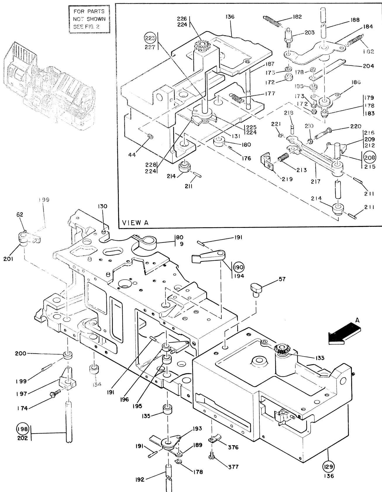
FIGURE 13. CARD TRANSPORT ASMS FOR STD, STD/HSS, STD/IGP AND S.C. FEATURES. SHEET 7 OF 7. SEE LIST 13.
