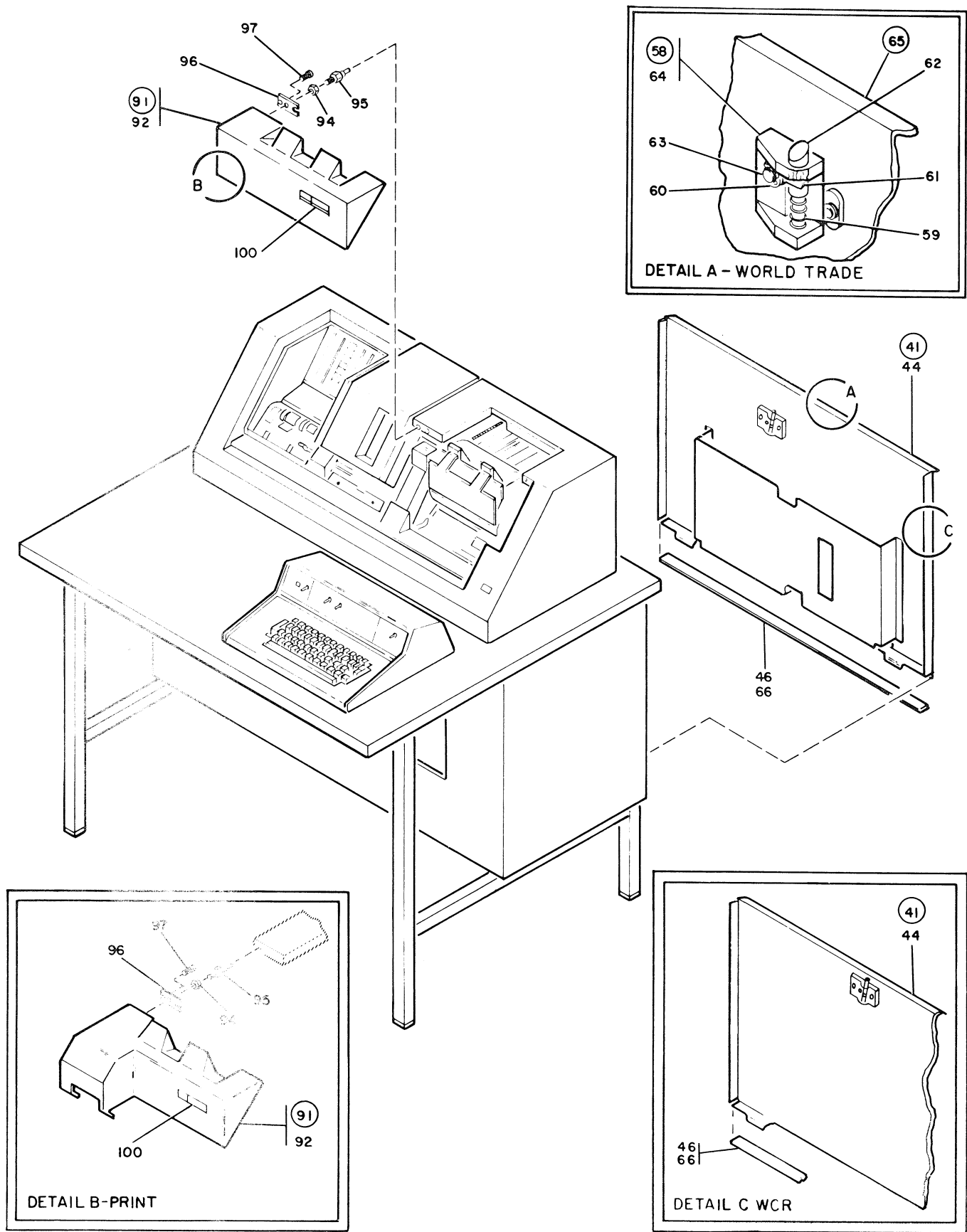
FIGURE 1. STANDARD AND FEATURE COVER ASSEMBLIES. SHEET 1 OF 2. SEE LIST 1.
