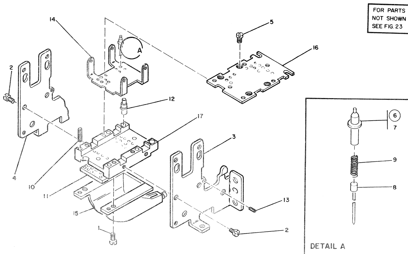
FIGURE 24. PRINT WIRE UNIT ASSEMBLY. SEE LIST 24.
