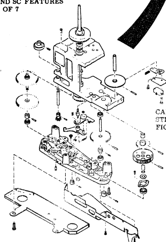
CARD TRANSPORT ASMS FOR STD, STD/HSS, STD/IGP AND SC FEATURES FIGURE 13, SHEET 2 OF 7
