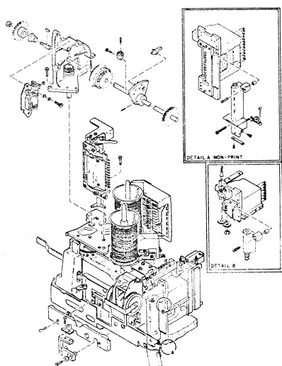
CARD TRANSPORT ASMS FOR VLCD, VLCD/HSS AND SELF CHECK FEATURE FIGURE 14, SHEET 2 OF 7
