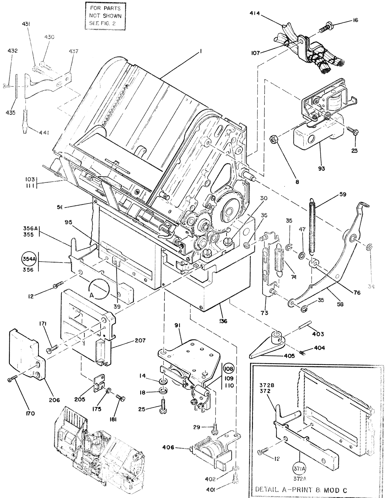
FIGURE 13. CARD TRANSPORT ASMS FOR STD, STD/HSS, STD/IGP AND S.C. FEATURES. SHEET 6 OF 7. SEE LIST 13.
