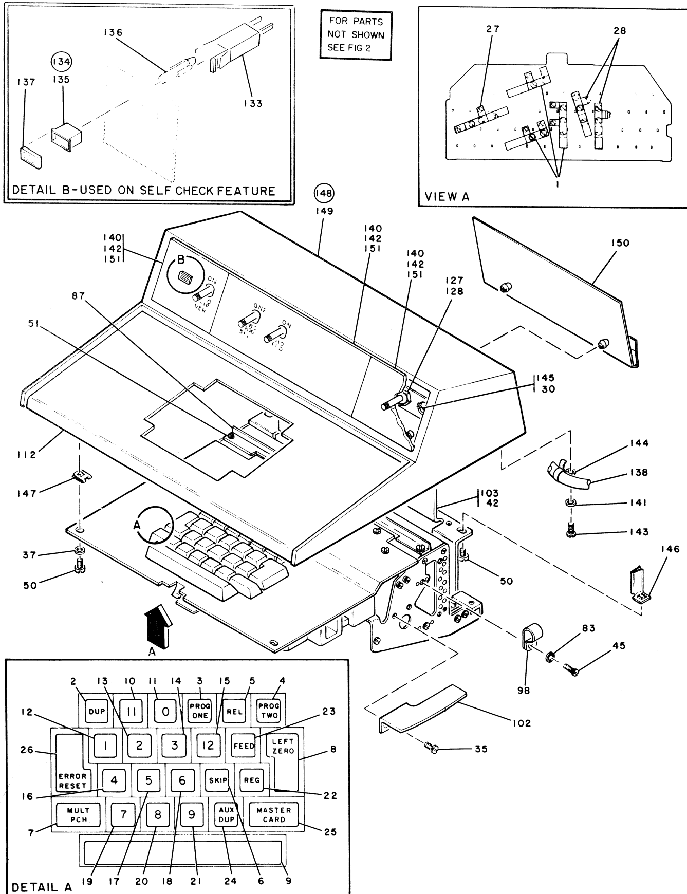
FIGURE 4. NUMERIC KEYBOARD AND COVER ASSEMBLIES. SHEET 1 OF 4. SEE LIST 4.
