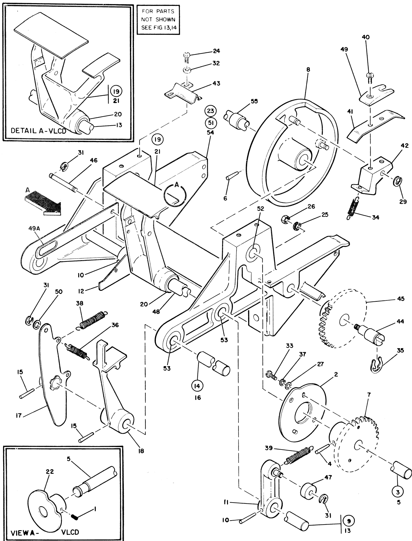
FIGURE 17. STANDARD AND FEATURE STACKER ASSEMBLIES. SEE LIST 17.
