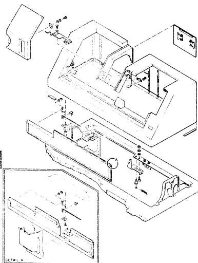
STANDARD AND FEATURE COVER ASSEMBLIES FIGURE 1, SHEET 2 OF 2
