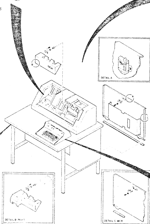
STANDARD AND FEATURE COVER ASSEMBLIES FIGURE 1, SHEET 1 OF 2
