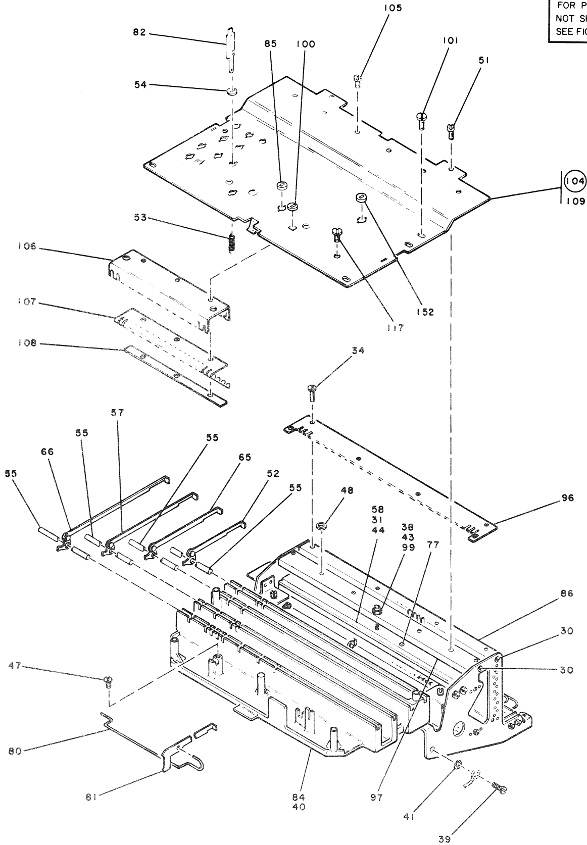
FIGURE 5. COMBINATION KEYBOARDS AND COVER ASSEMBLIES. SHEET 2 OF 5. SEE LIST 5.
