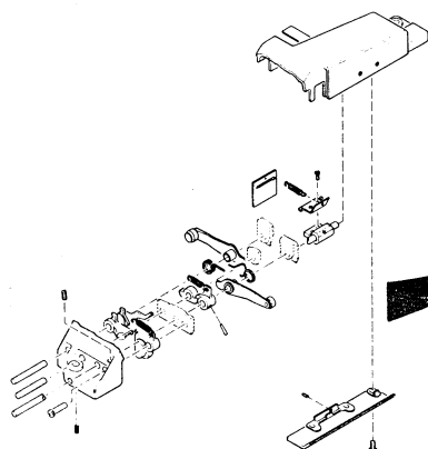
UNIT EJECT ASSEMBLIES FIGURE 32
