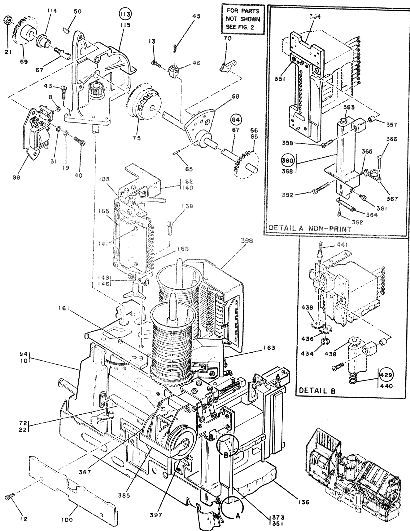
FIGURE 13. CARD TRANSPORT ASMS FOR STD, STD/HSS, STD/IGP AND S.C. FEATURES. SHEET 2 OF 7. SEE LIST 13.
