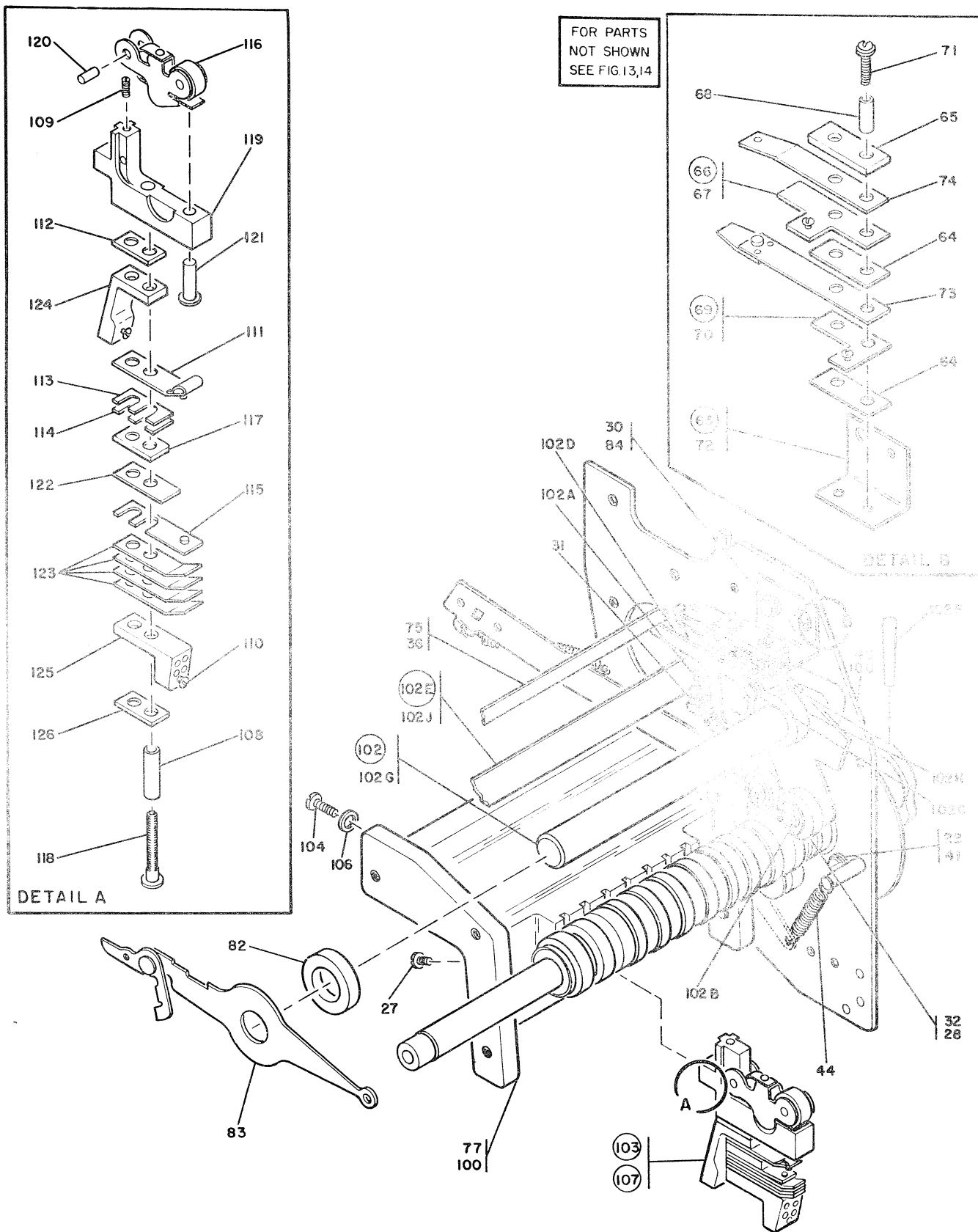
FIGURE 33. MAGNET AND PUNCH DRIVE ASSEMBLIES. SHEET 2 OF 3. SEE LIST 33.
