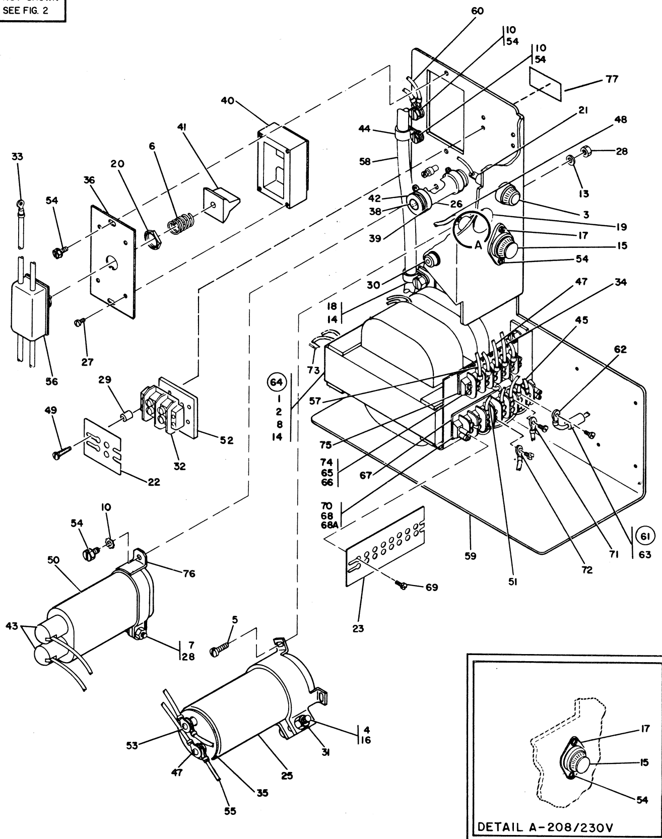
FIGURE 50. MODEL C 50 AND 60 CYCLE POWER SUPPLY ASSEMBLIES. SEE LIST 50
