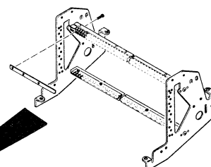
MOUNTING BAR ASSEMBLY FIGURE 6
