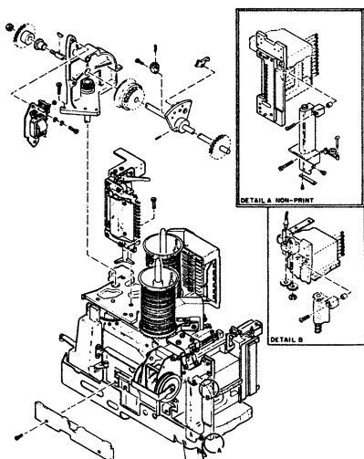
CARD TRANSPORT ASMS FOR STD, STD/HSS, STD/IGP AND SC FEATURES FIGURE 13, SHEET 2 OF 7
