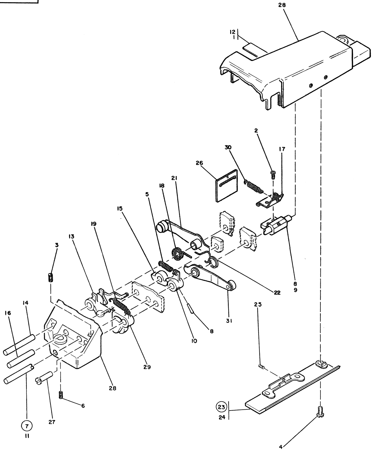
FIGURE 32. UNIT EJECT ASSEMBLIES. SEE LIST 32.
