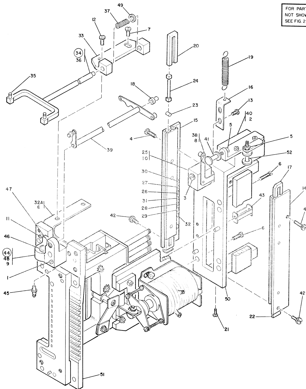
FIGURE 27. INTERPRETER INTERPOSER AND PUNCH ASSEMBLY. SEE LIST 27.
