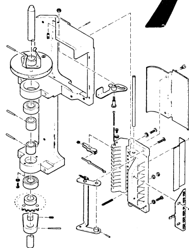
AUXILIARY UNIT SENSING ASSEMBLY FIGURE 37
