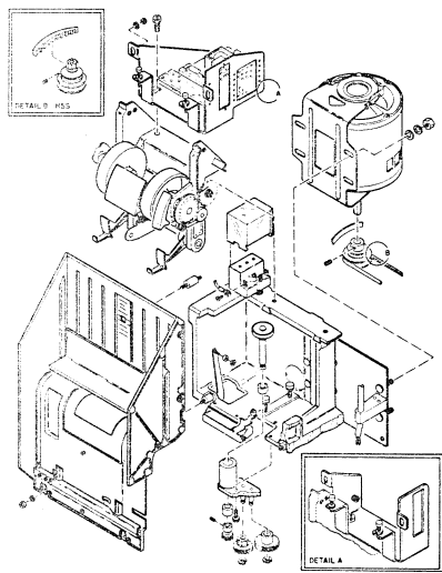
CARD TRANSPORT ASMS FOR VLCD, VLCD/HSS AND SELF CHECK FEATURE FIGURE 14, SHEET 1 OF 7
