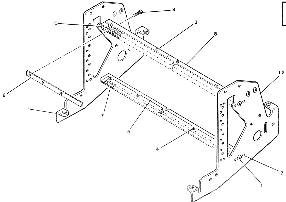
FIGURE 6. MOUNTING BAR ASSEMBLY. SEE LIST 6.
