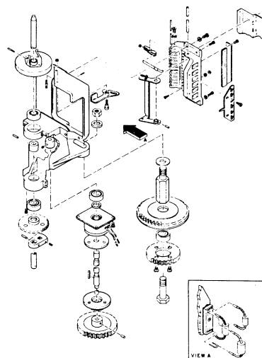
HIGH SPEED SKIP CLUTCH ASSEMBLY WITH SENSING FOR AUXILIARY DUPLICATION FIGURE 36
