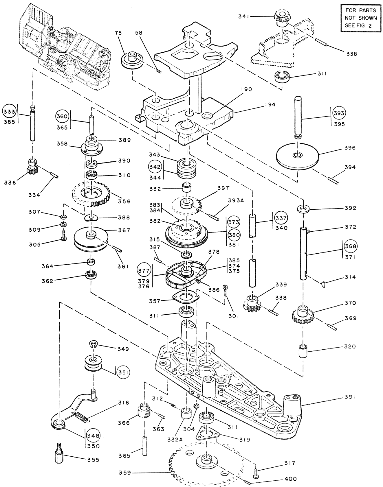
FIGURE 14. CARD TRANSPORT ASSEMBLIES FOR VLCD, VLCD/HSS AND SELF CHECK FEATURE. SHEET 5 OF 7. SEE LIST 14.
