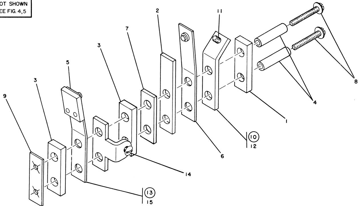
FIGURE 12. ALPHA, PROGRAM 2, FEED AND DUP KEYS CONTACT ASSEMBLY. SEE LIST 12
