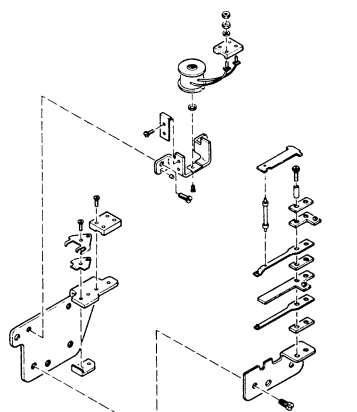
ESCAPEMENT MAGNET ASSEMBLY FIGURE 40
