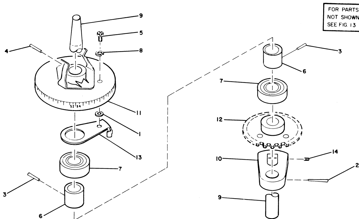
FIGURE 30. PROGRAM DRUM SHAFT ASSEMBLY. SEE LIST 30.
