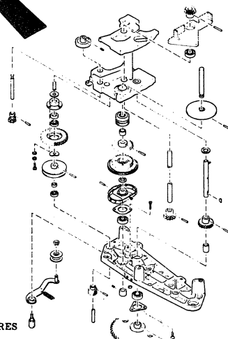
CARD TRANSPORT ASMS FOR STD, STD/HSS, STD/IGP AND SC FEATURES FIGURE 13, SHEET 7 OF 7
