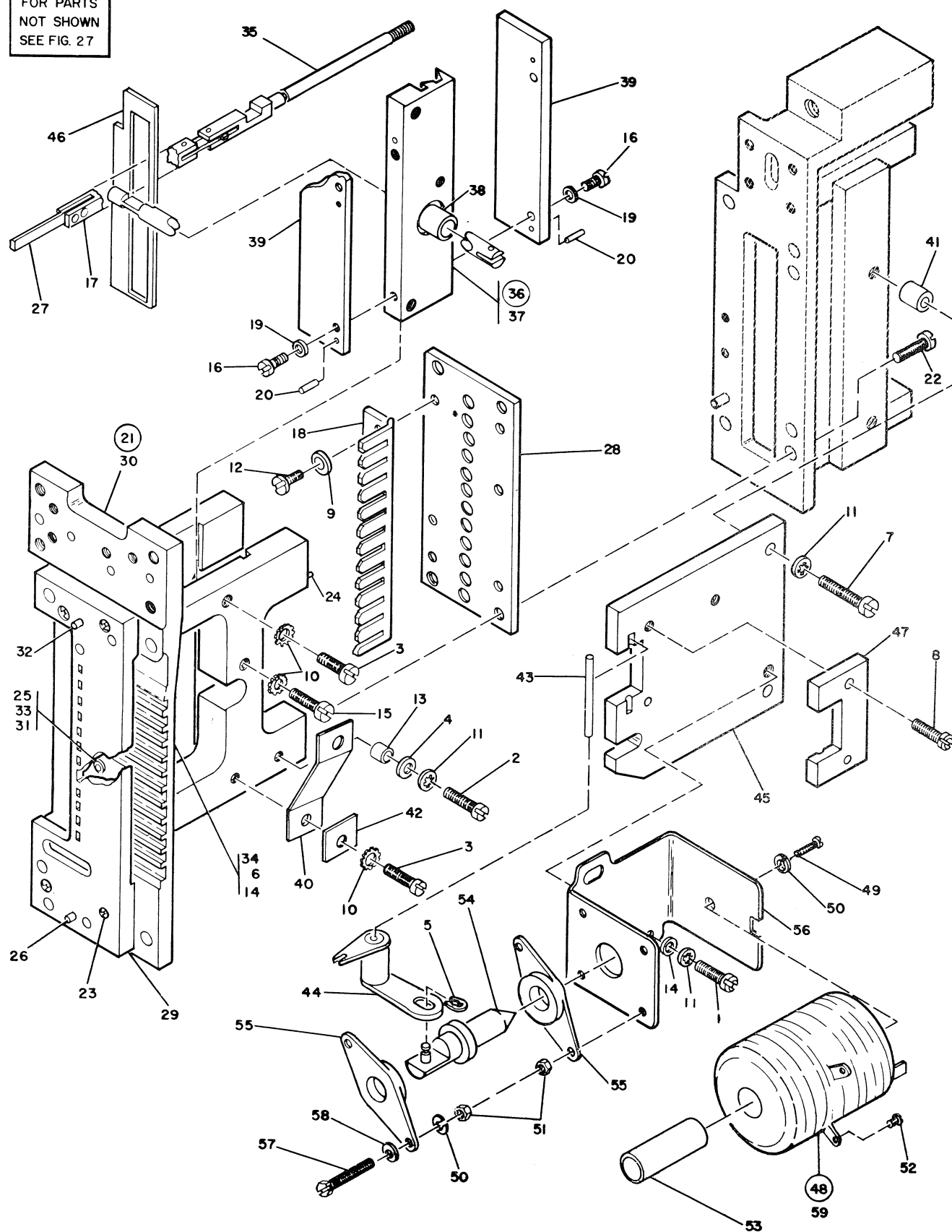
FIGURE 28. INTERPRETER PUNCH ASSEMBLY. SEE LIST 28.
