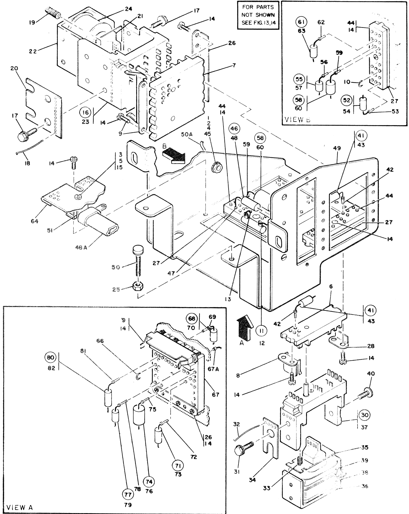
FIGURE 39. STACKER MOUNTING BRACKET AND TERMINAL BLOCK ASSEMBLY. SEE FIG. 13, 14
