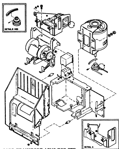
CARD TRANSPORT ASMS FOR STD, STD/HSS, STD/IGP AND SC FEATURES FIGURE 13, SHEET 1 OF 7
