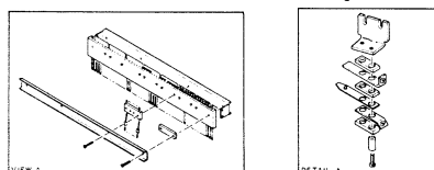
COMBINATION KEYBOARDS AND COVER ASSEMBLIES FIGURE 5, SHEET 2 OF 5
