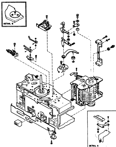
CARD TRANSPORT ASMS FOR STD, STD/HSS, STD/IGP AND SC FEATURES FIGURE 13, SHEET 3 OF 7
