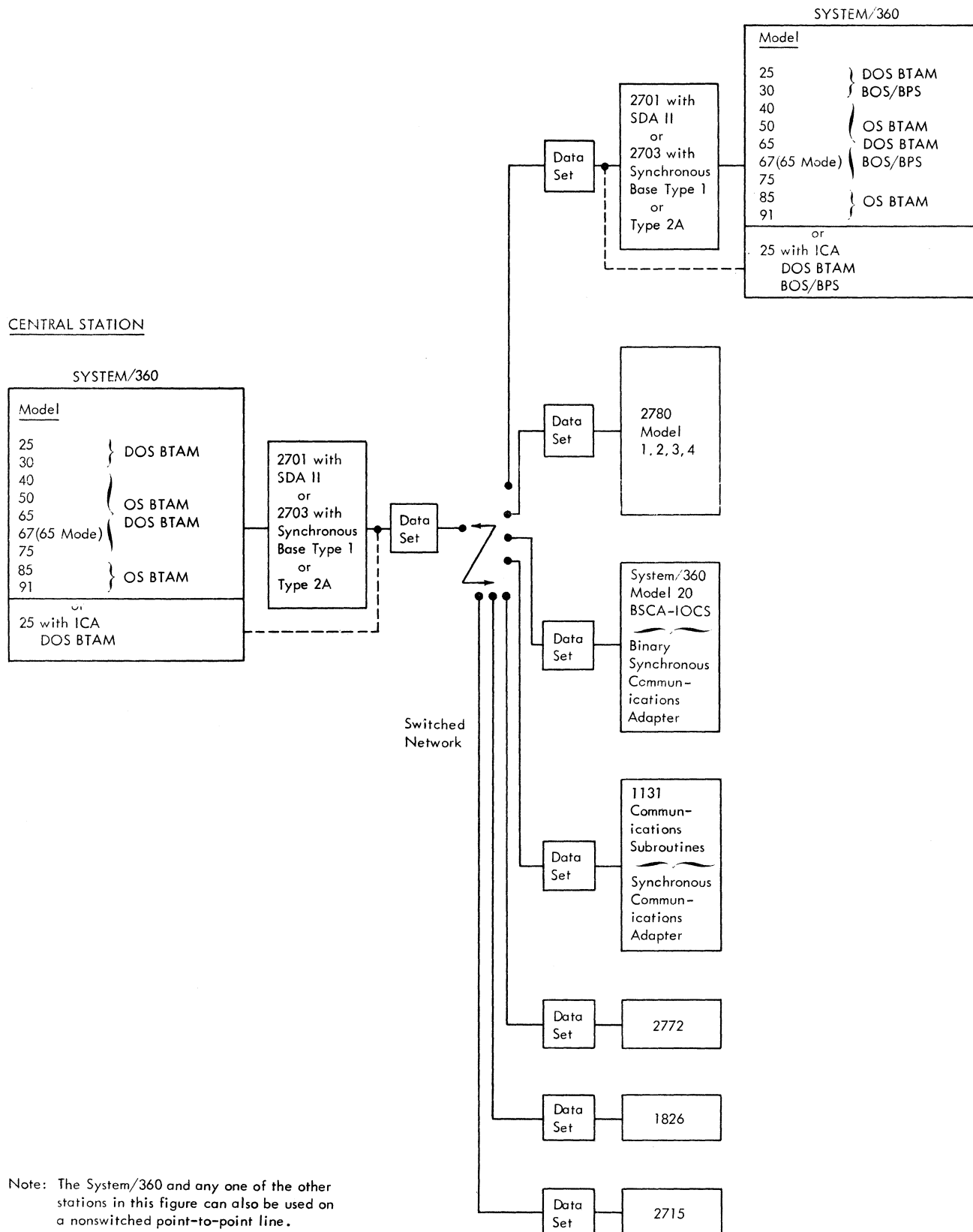
Figure 23. BSC Intermix-Switched Point-to-Point
