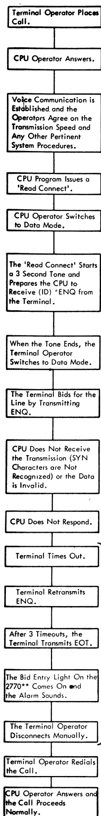
Figure 29. Transmission Fails to Start—Manual Answer (2770 or 2780-to-System/360)
