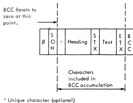
Figure 8. Block Check Character Accumulation—Entire Transmission
