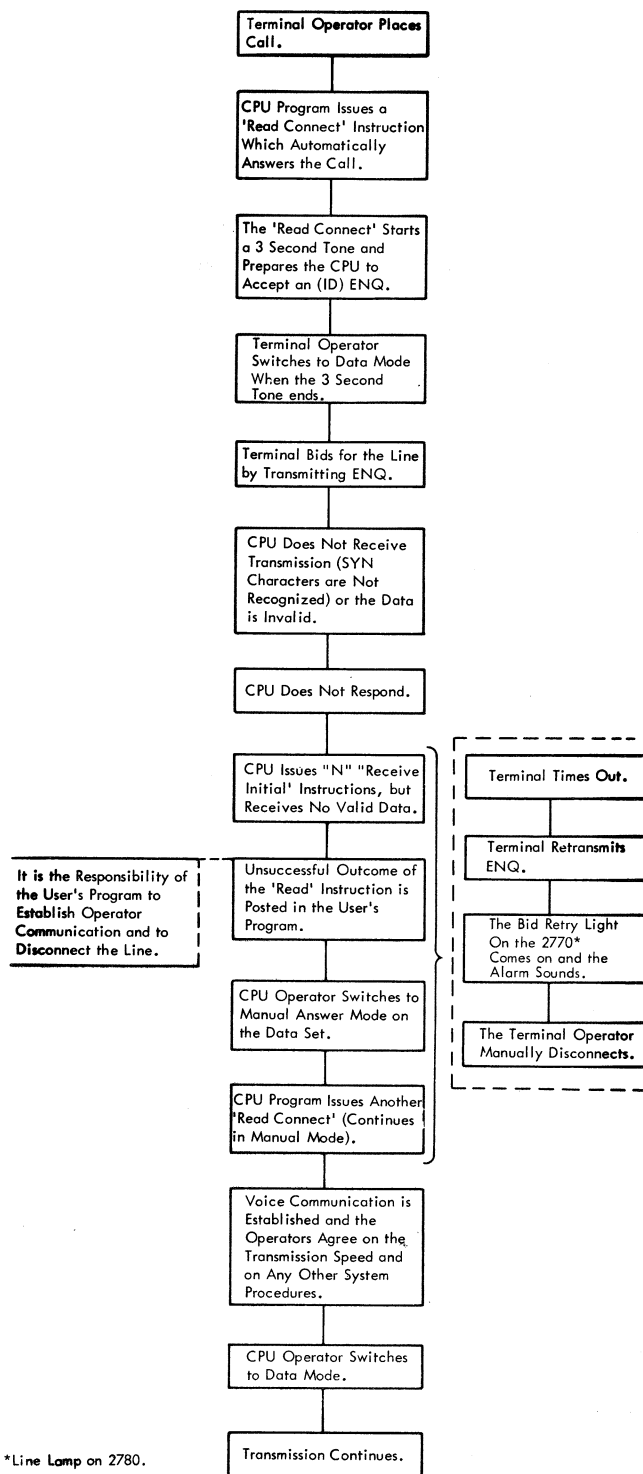
Figure 30. Transmission Fails to Start—Automatic Answer (2770 or 2780-to-System/360)
