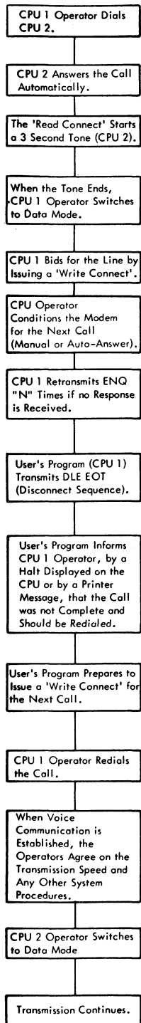
Figure 27. Transmission Fails to Start (System/360-to-System/360)
