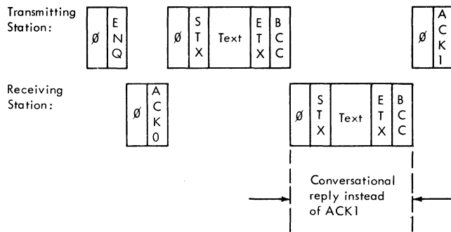
Figure 18. Limited Conversational Mode
