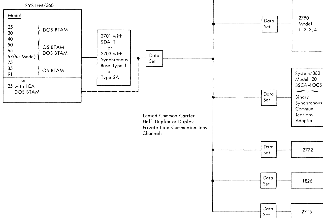
Figure 22. BSC Intermix-Multipoint
