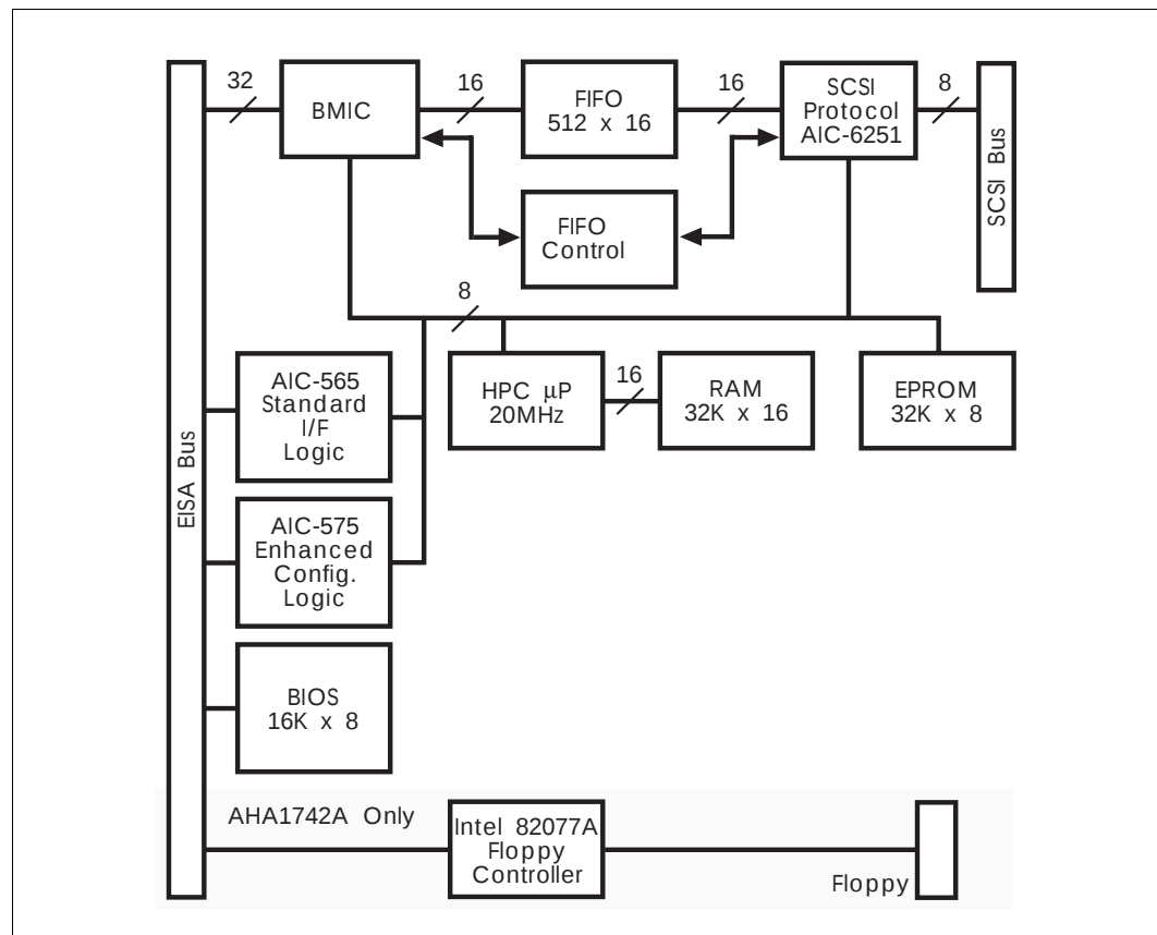
Figure 2-1. AHA-1740A/1742A Block Diagram
