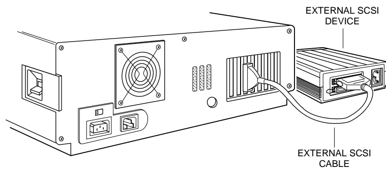
Figure 2-10. Connecting External Cable to SCSI Device
