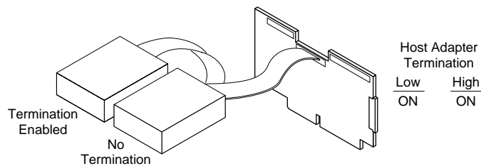
Figure 2-4. Internal Wide SCSI Devices Only
