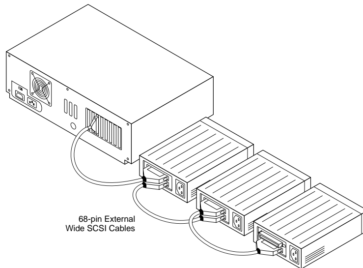
Figure 2-18. Connecting Multiple External Wide SCSI Devices
