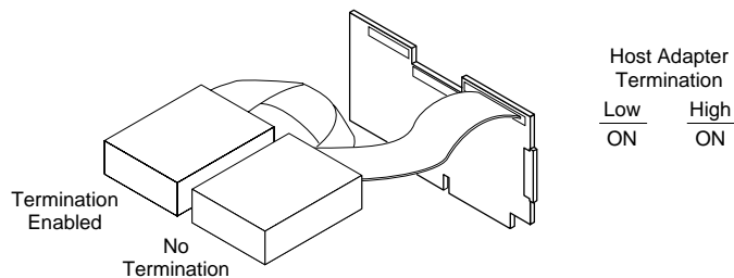
Figure 2-7. Internal 8-bit SCSI Devices Only
