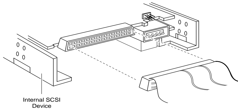
Figure 2-14. 68-pin Internal Cable to Internal Wide SCSI Device
