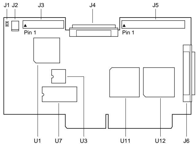
Figure 1-1. Board Layout for the AHA-2740W and AHA-2742W
