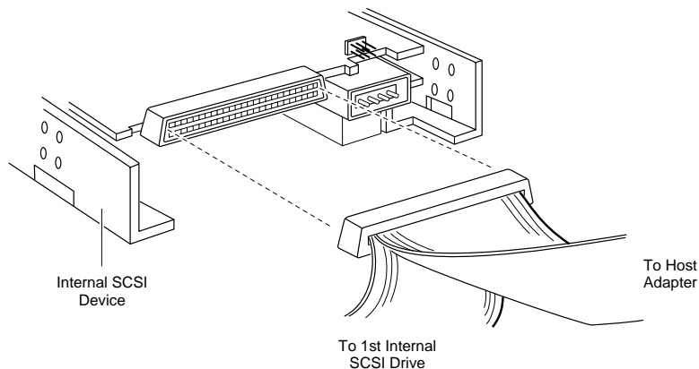
Figure 2-15. Connecting a Second Internal Wide SCSI Device
