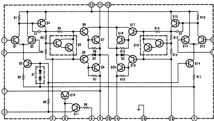
μPC 1490HA BLOCK DIAGRAM
