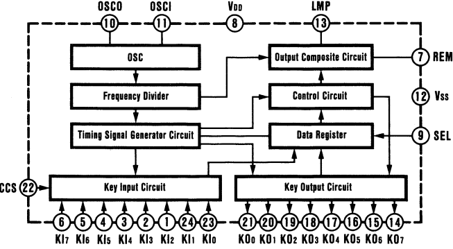
TC 9148P BLOCK DIAGRAM
