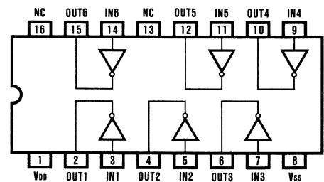
LC 4049 BLOCK DIAGRAM
