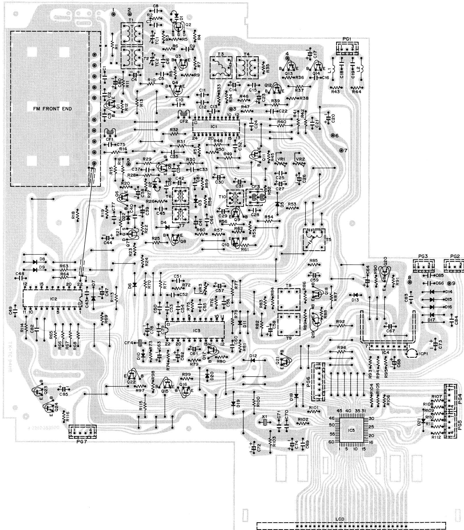
TUNER PRINTED CIRCUIT BOARD (BOTTOM VIEW)
