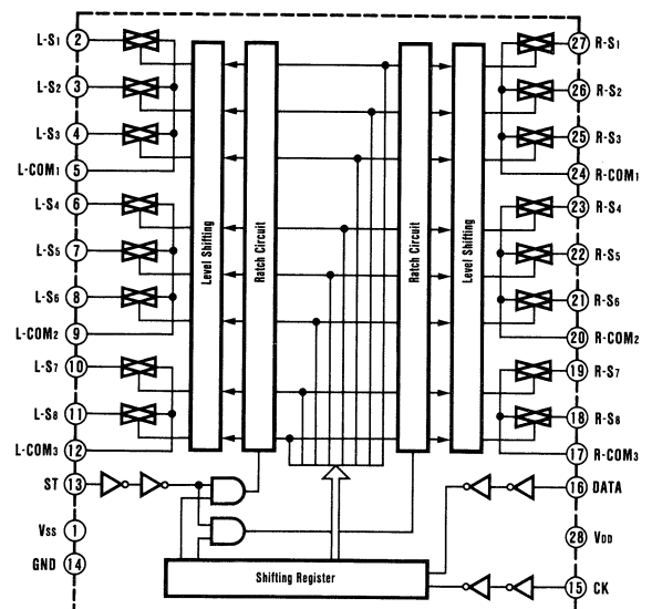
TC 9163N BLOCK DIAGRAM
