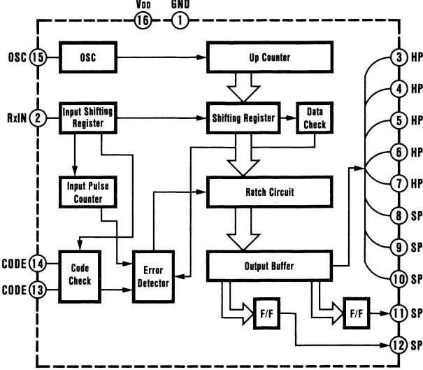
TC 9149P BLOCK DIAGRAM
