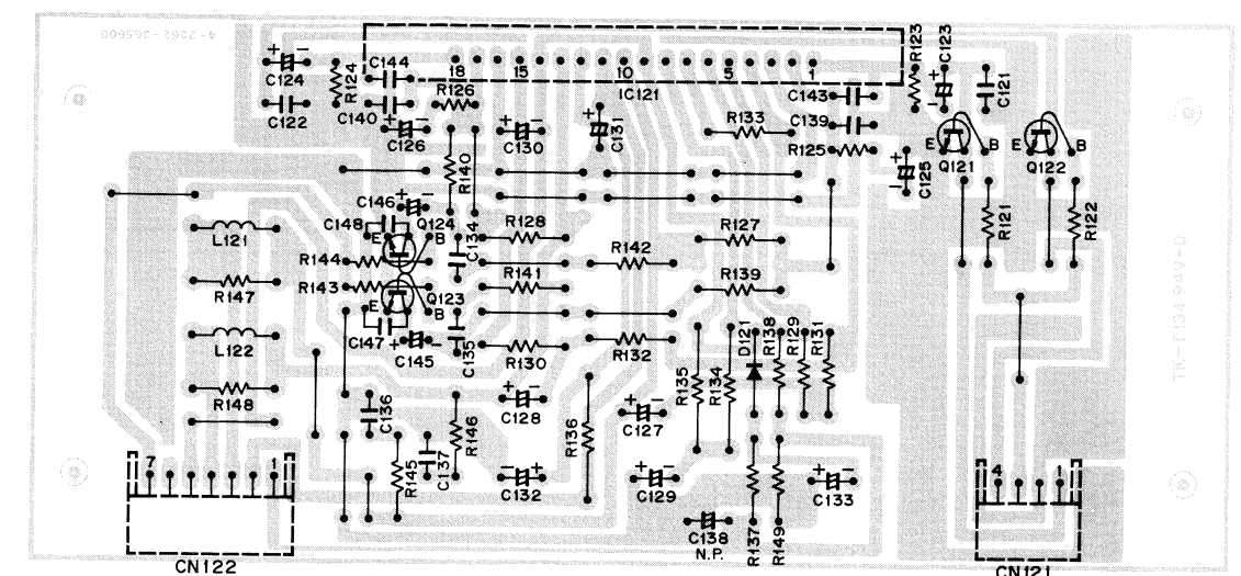
POWER AMP P.C.BOARD (BOTTOM VIEW)
