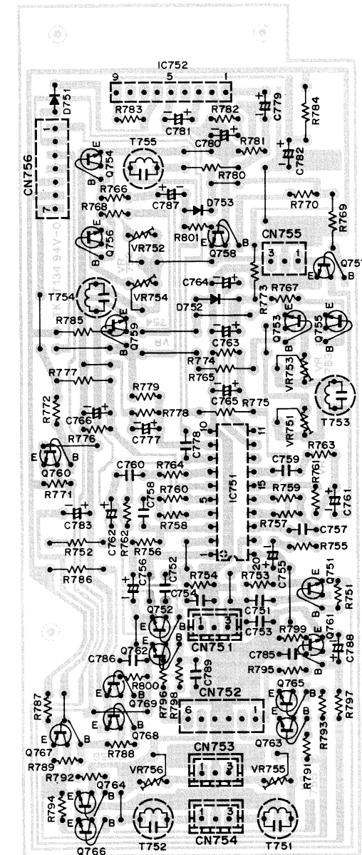
POWER AMP P.C.BOARD (BOTTOM VIEW)
