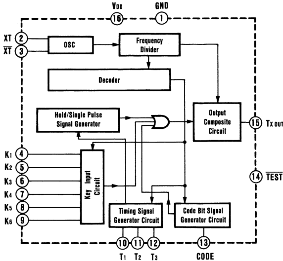
TC 9148P BLOCK DIAGRAM
