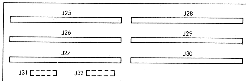
(b) CONNECTOR LAYOUT OF I/O GROUNDPLANE
