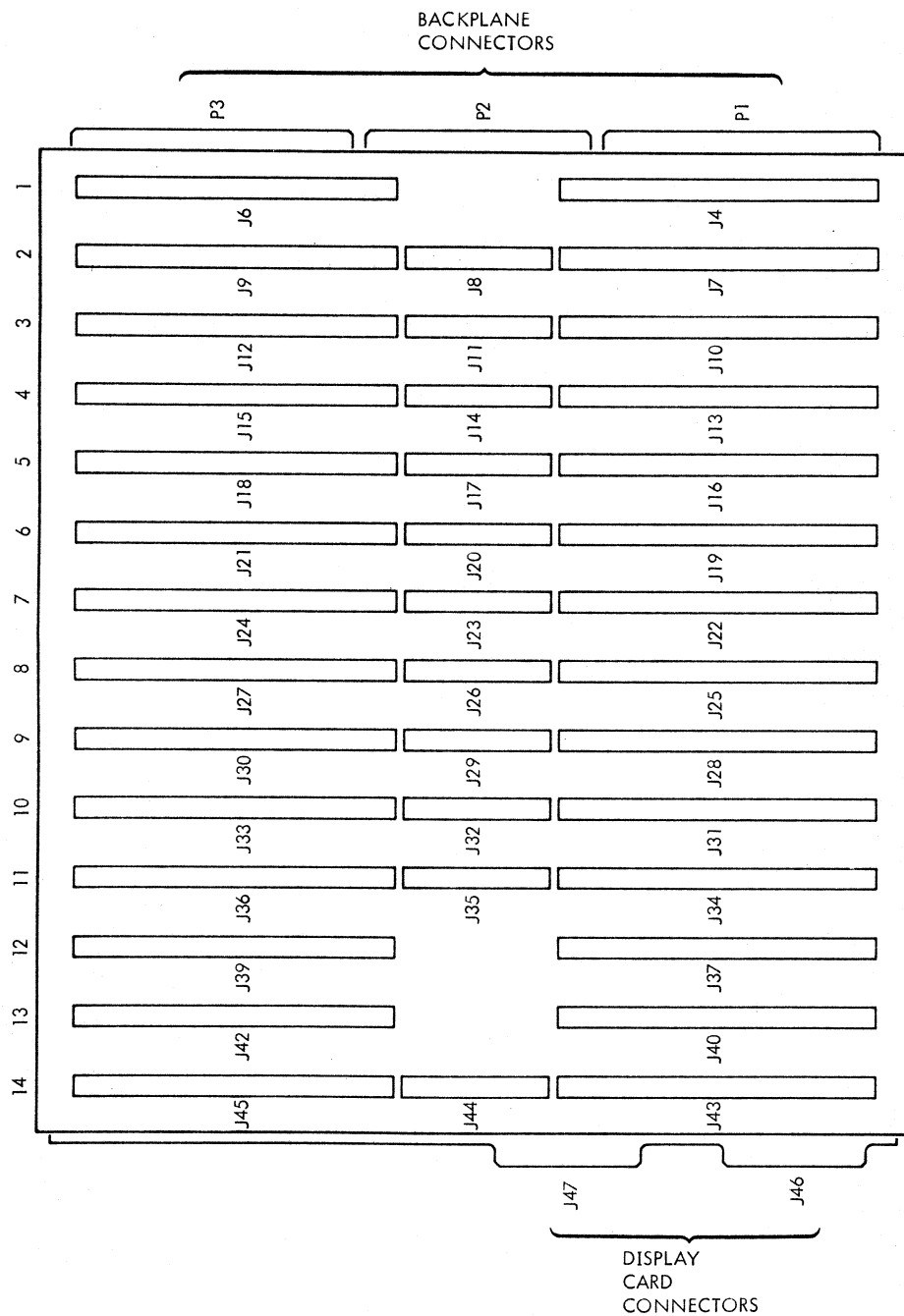
Figure II-2. Top View of CPU Tray
