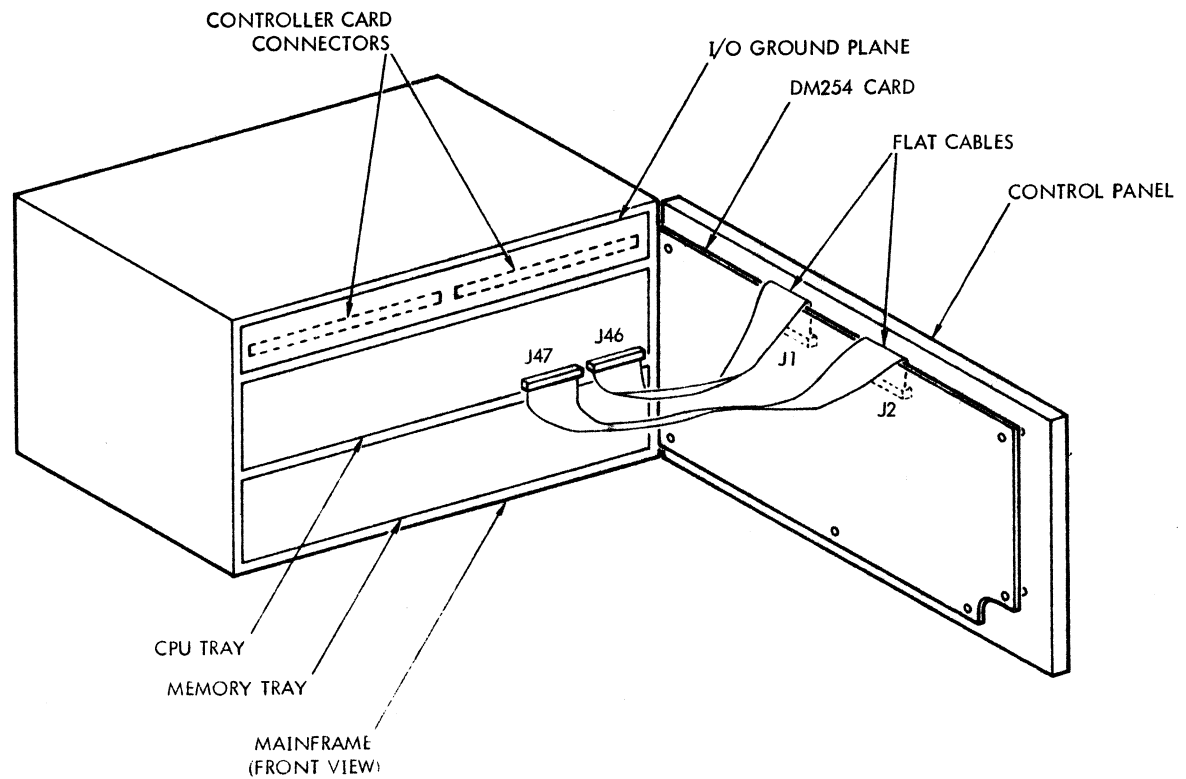
Figure II-1. Mainframe With Open Control Panel
