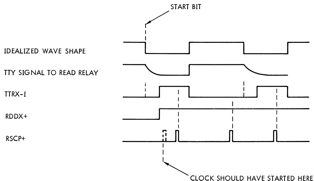
Figure 5-1. Shift Clock Pulse (RSCP +) Delay Adjustment
