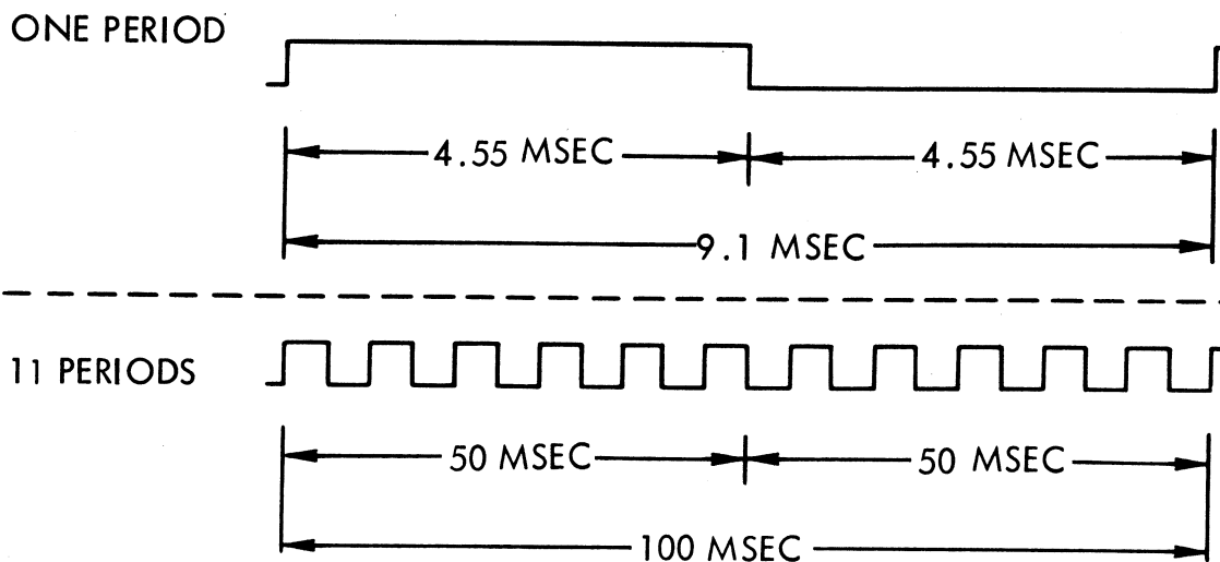
Figure 5-4. Waveforms for Transmit Clock Adjustment
