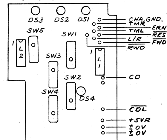
COMPONENT LAYOUT 6013
