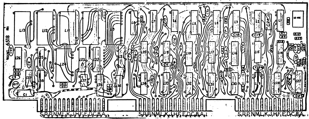
COMPONENT LAYOUT
