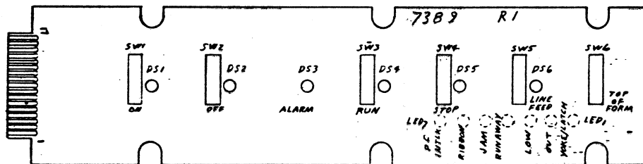
COMPONENT LAYOUT
