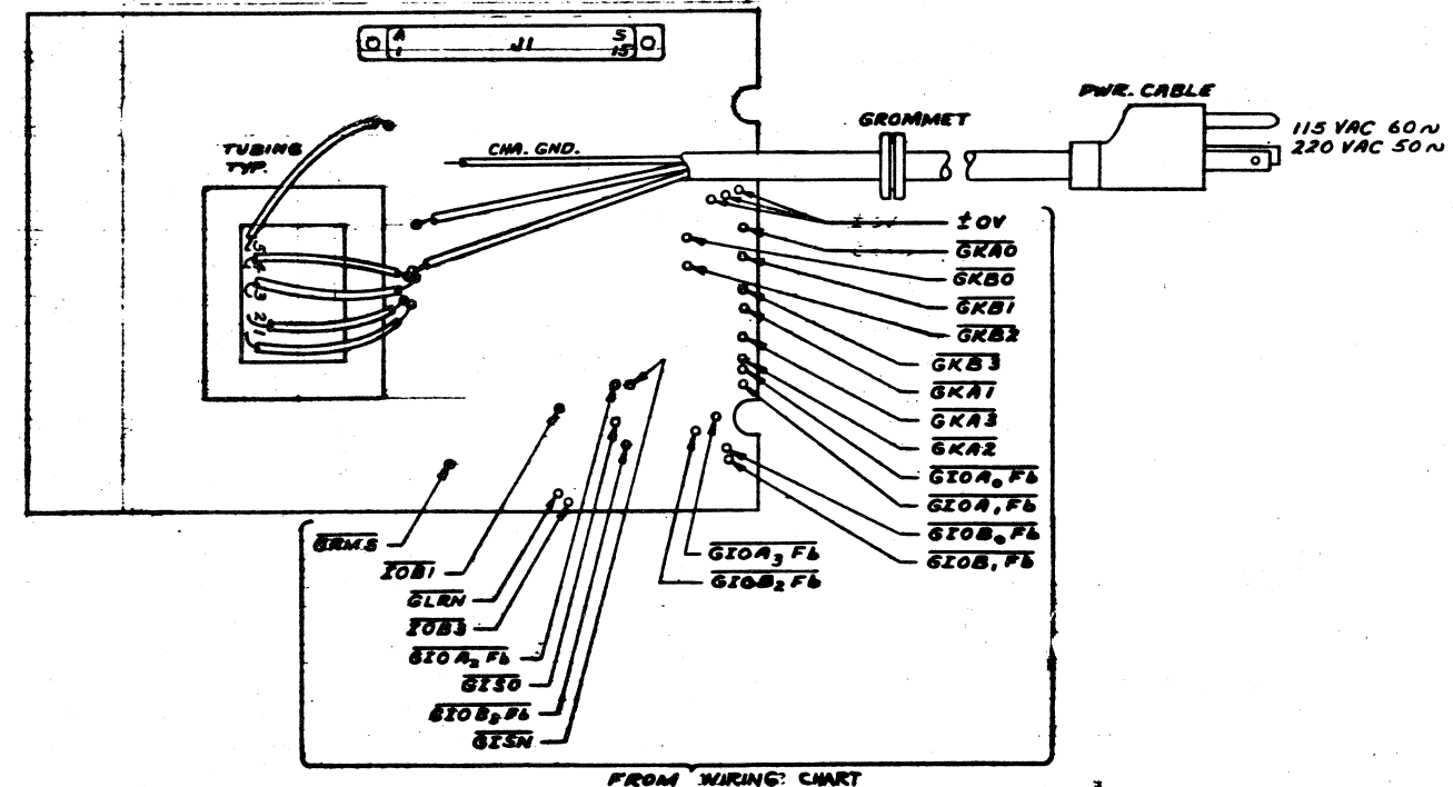
COMPONENT LAYOUT FOR 6127
