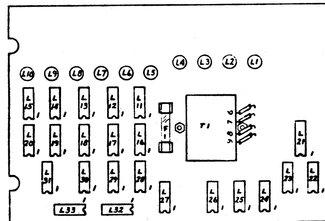
COMPONENT LAYOUT FOR 6127
