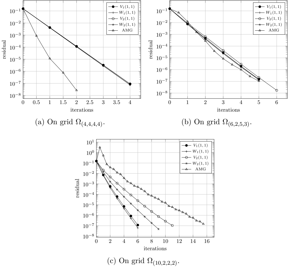
Figure 5.4: Convergence history for problem 1b with d = 4 .
