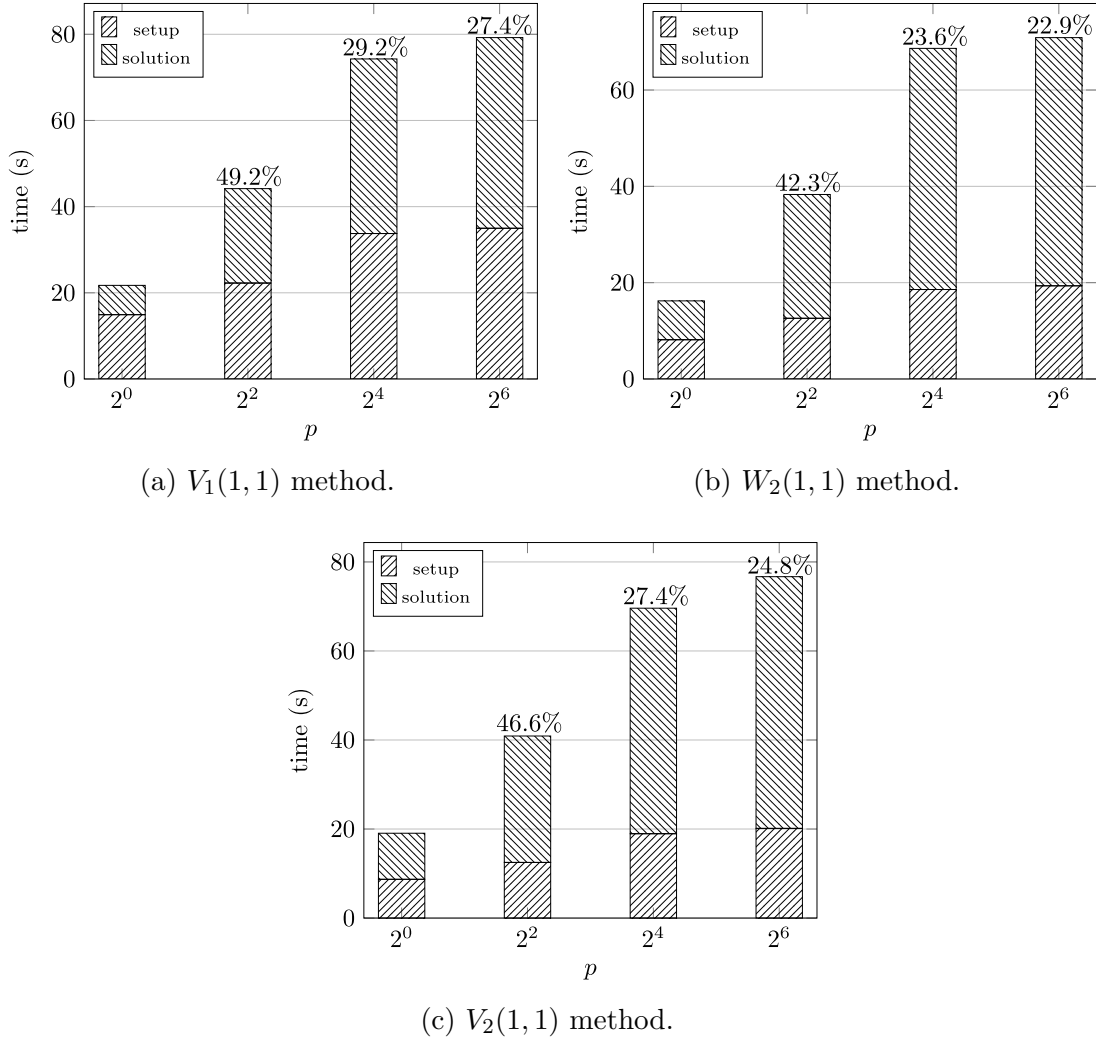
Figure 5.7: Weak scalability for problem 1b with d = 2 and \psi_l = 2^{14} . The weak scaling efficiency is given as percentage above the bars.
