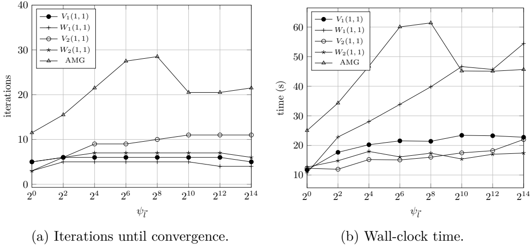
Figure 5.3: Behavior of multigrid methods for problem 1b with d = 2 and different aspect ratios.
