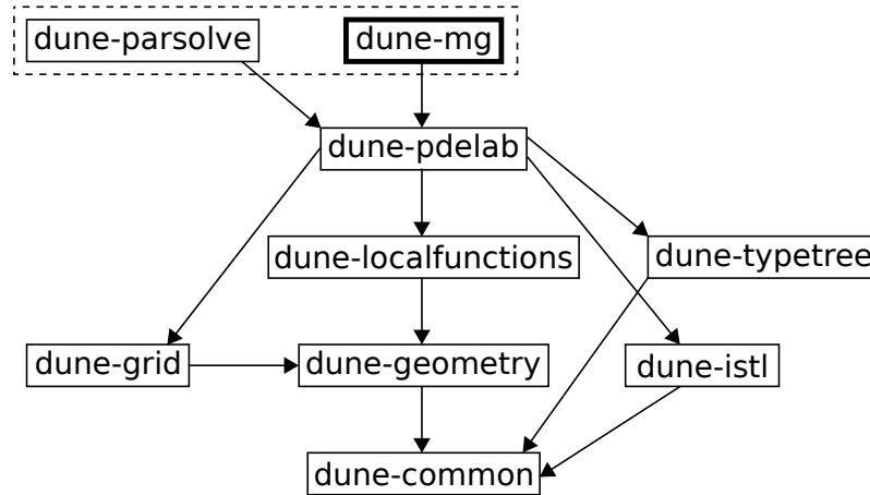
Figure 4.1: Dependency graph of the DUNE modules
