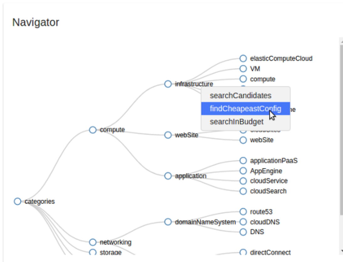
Figure 4.7.: Navigator View
