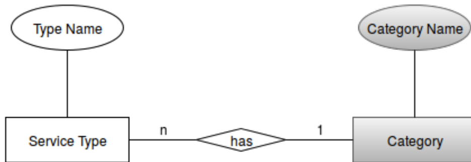
Figure 3.3.: Entity-Relation Diagram
