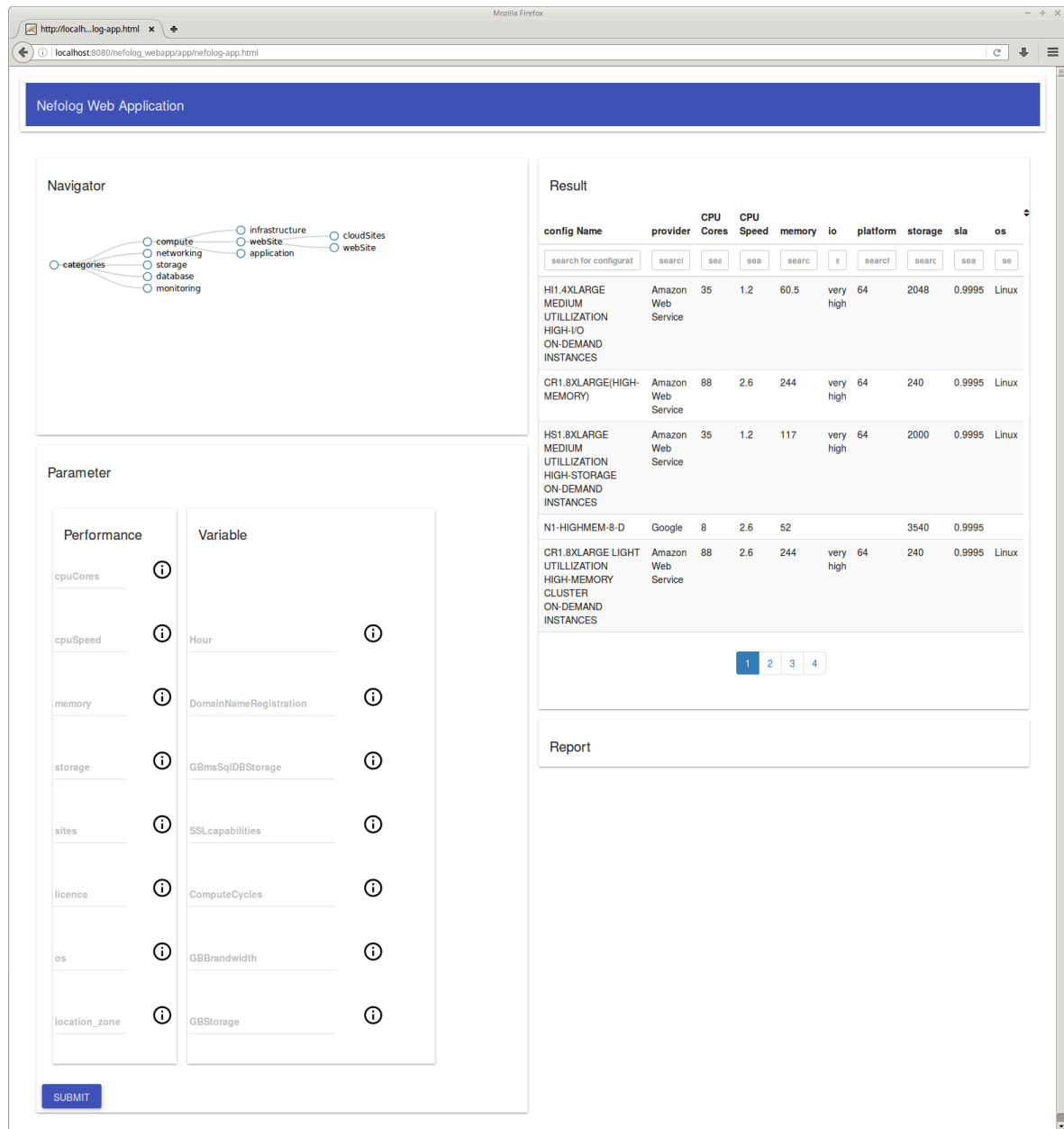
Figure 4.6.: Layout for User Interface
