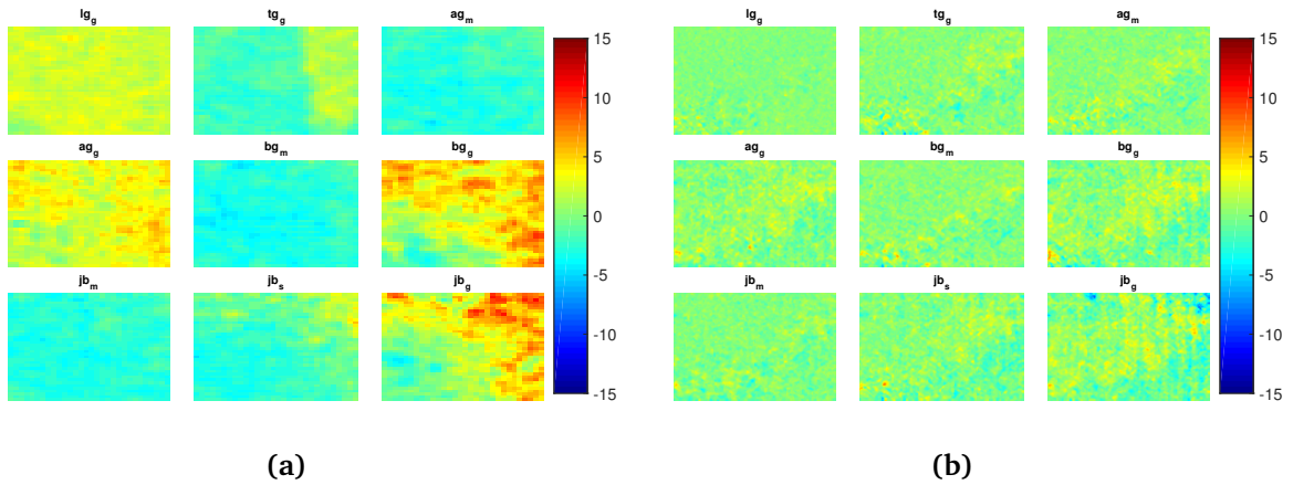
Figure 5.6: Difference images for Kinect ToF (a) and Ensenso N10 (b) at mid distance (Bottom left is closer to depth image center)
