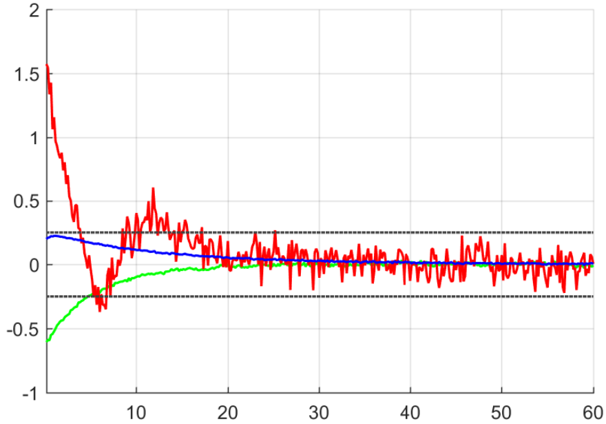
Figure 5.2: Deviation of average depth value [mm] during warm-up over 60 minutes Blue: Ensensio N10, Green: Kinect SL , Red: Kinect ToF
