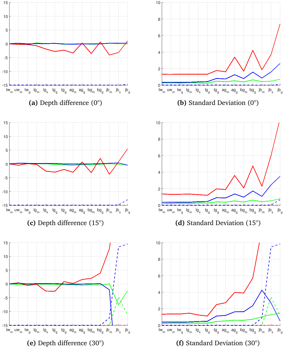
Figure 5.8: Difference to averaged depth value [mm] and average standard deviation [mm] of pixels between frames measured from 1m distance at 0^\circ , 15^\circ and 30^\circ . The ratio of invalid pixels is shown by the dashed lines. Blue: Ensenso N10, Green: Kinect SL , Red: Kinect ToF
