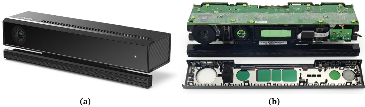
Figure 4.4: (a) Kinect for Windows v2 Sensor (Kinect ToF ) [Micb] and (b) opened casing revealing the IR-camera and light source sitting next to each other in the center of the device [iFi]
