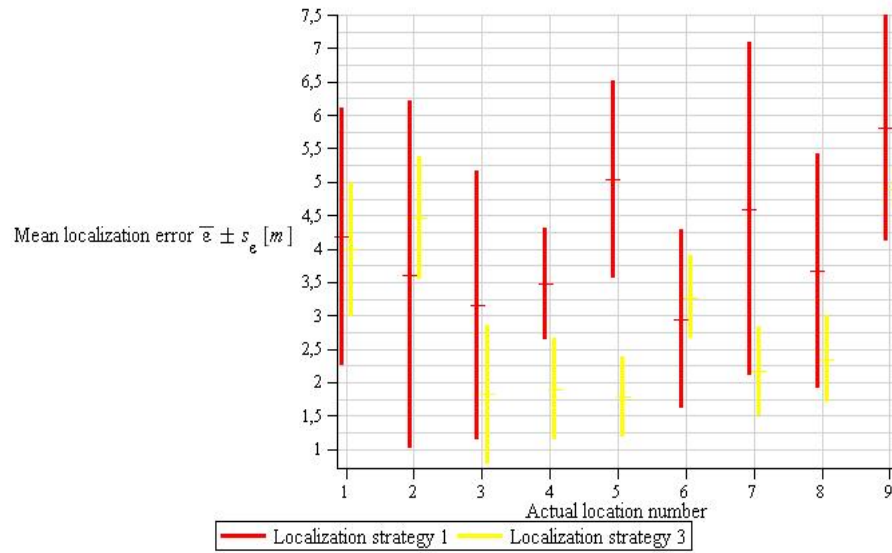
Figure 5.11: Performance of localization strategies 1 and 3 tested in the second session of experiments
