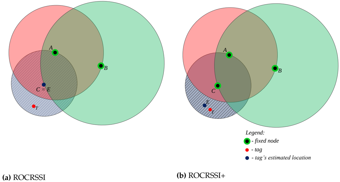
Figure 3.3: Difference between ROCRSSI and ROCRSSI+ while considering the area outside of the determined circles
