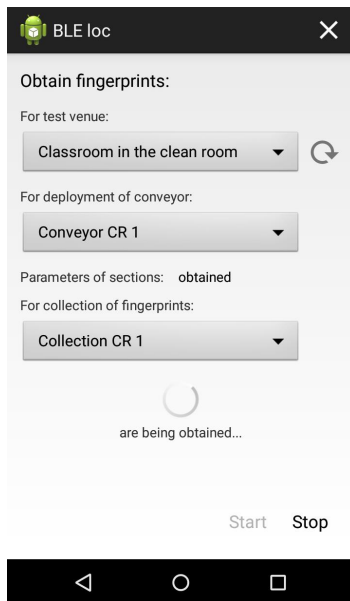
Figure 4.5: Android client application GUI – acquisition of fingerprints
