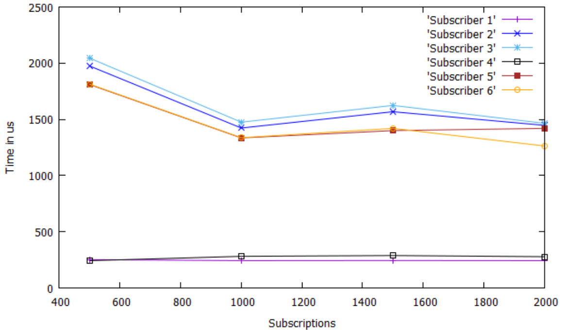
Figure 5.3: Hybrid System Delays
