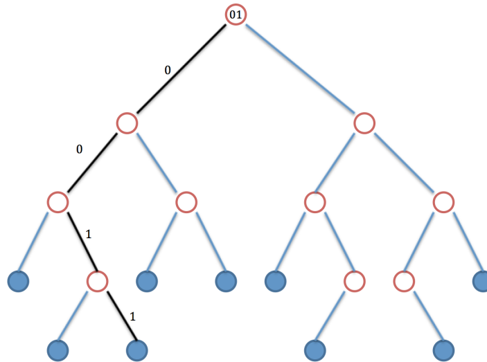
Figure 4.5: Event Matching
