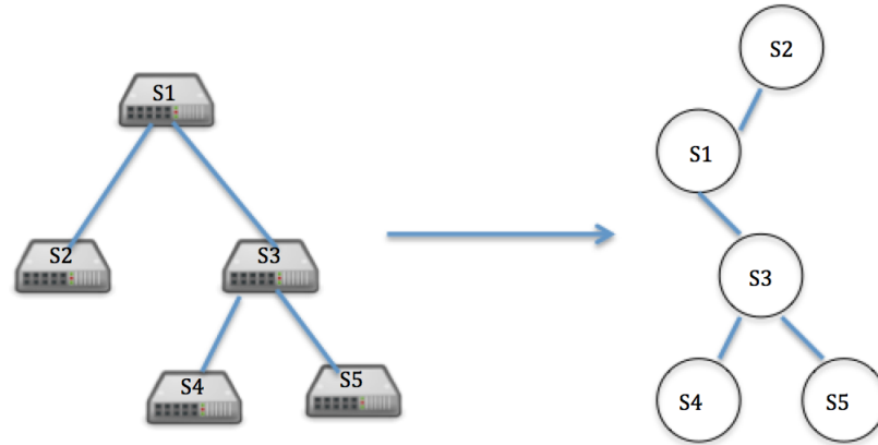
Figure 3.5: Spanning Tree
