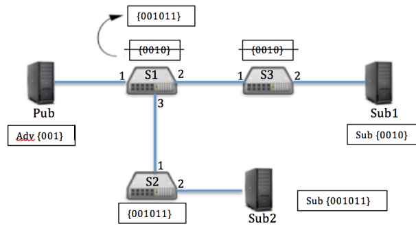
Figure 3.12: Un-Subscription
