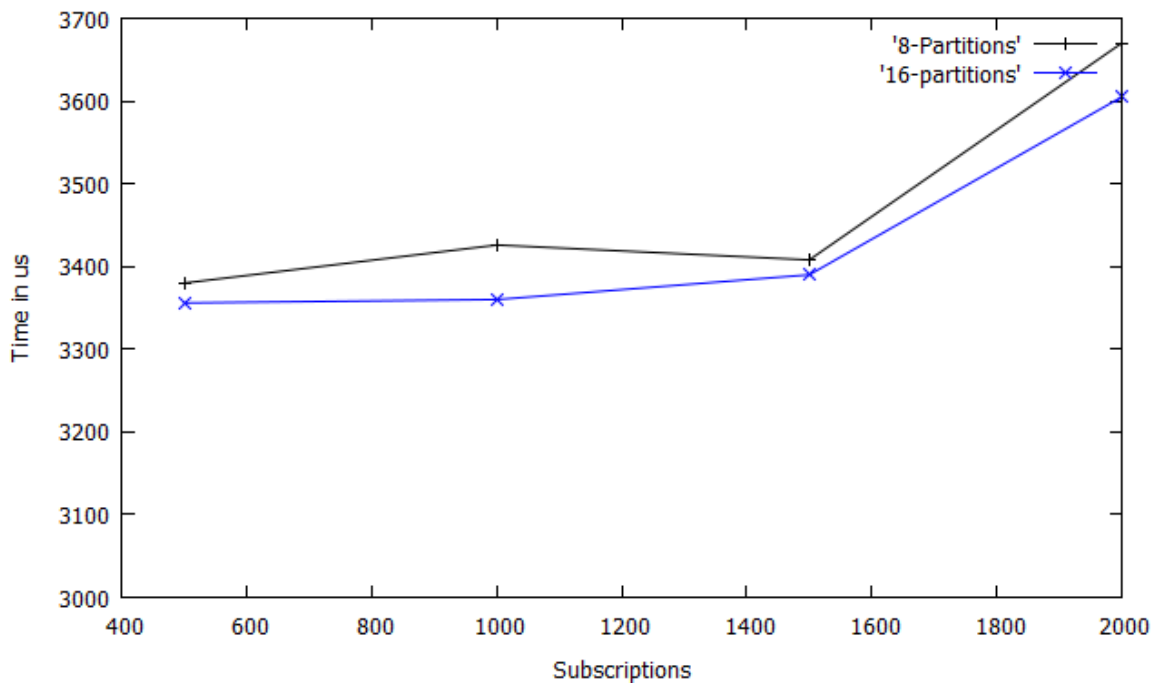
Figure 5.5: Performance Comparison
