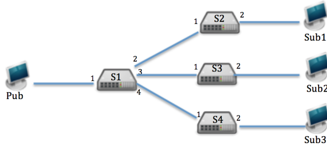
Figure 4.7: Mutual Forwarding
