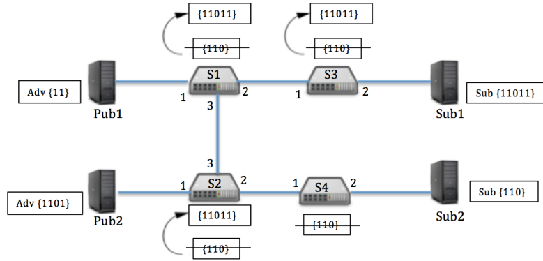
Figure 3.11: Un-Advertisement
