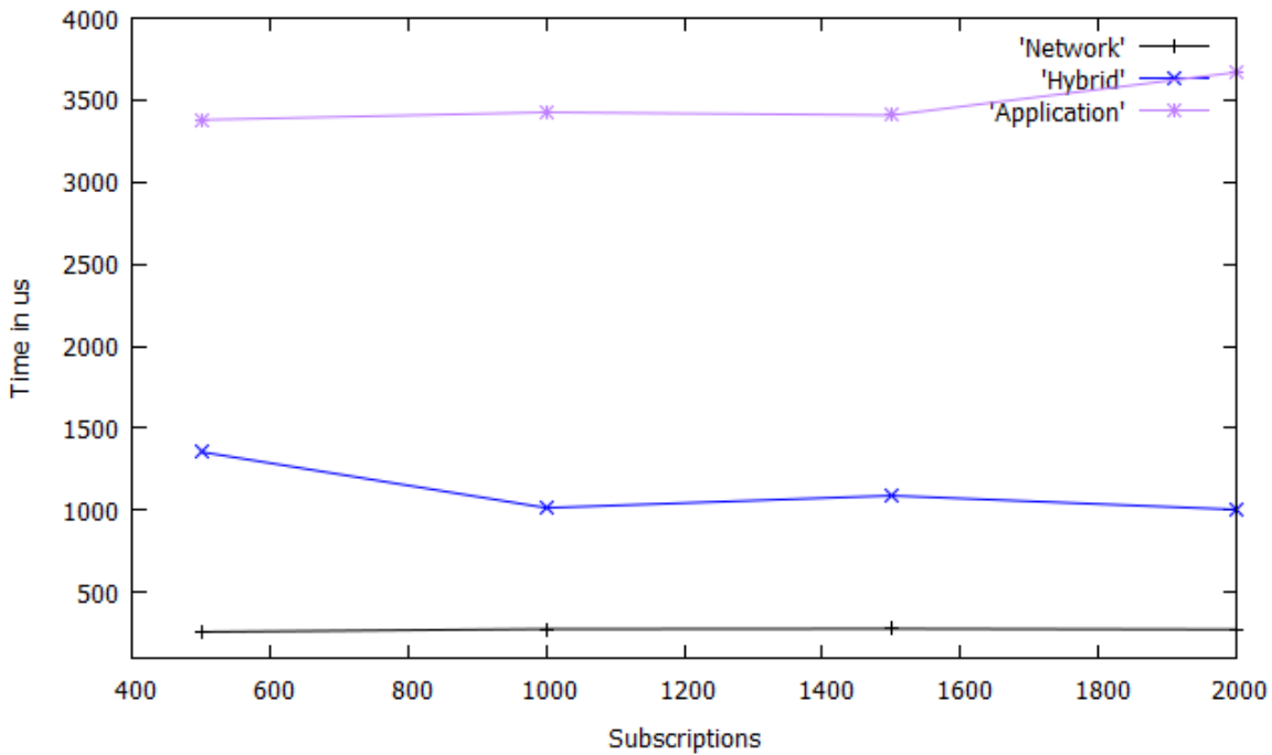
Figure 5.4: Delay Comparison
