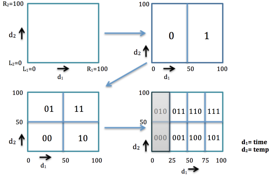
Figure 3.4: Spatial Indexing
