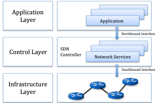
Figure 3.1: The SDN Architecture
