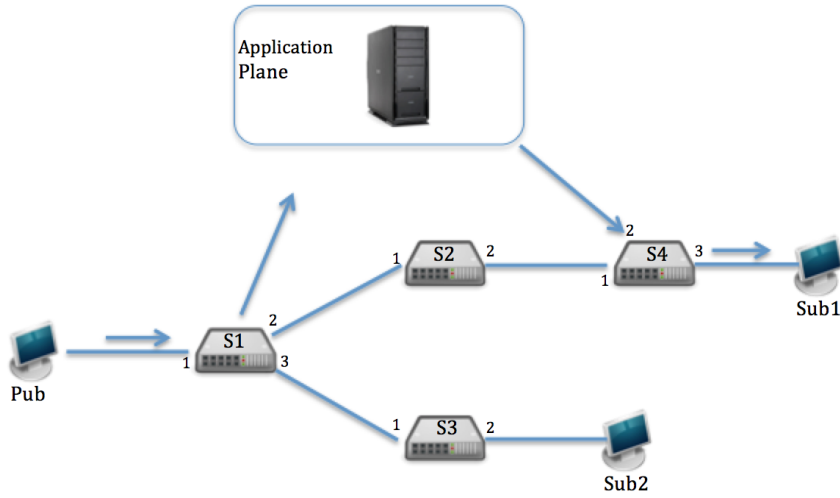
Figure 4.6: Direct Forwarding
