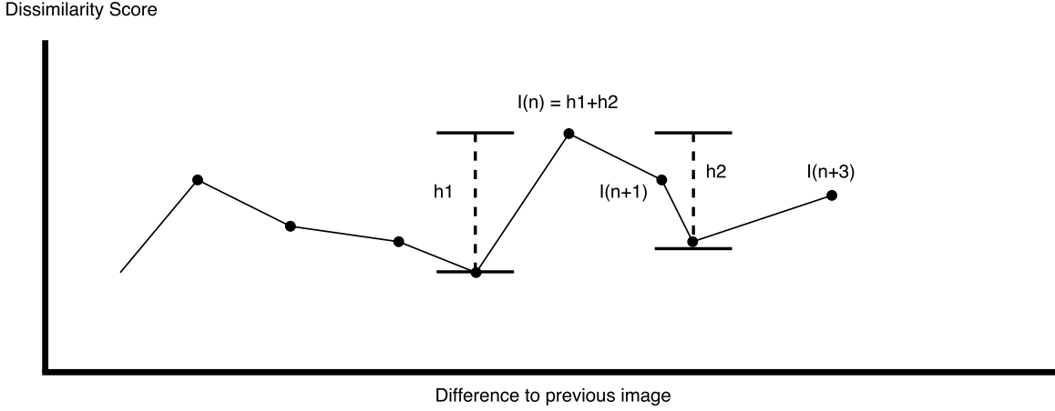
Figure 5.4.: Idea behind approaches that uses a peak in change to trigger event changes. The idea is to plot changes from image n to image n+1 and find the maximal turning point (here indicated through I(n) ). Image as shown in [DS08a].
