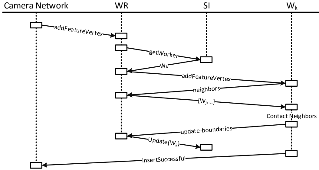
Figure 4.4: A detailed overview of the messages being sent and processed during an insert-operation of a vertex in the Master-Slave architecture. The nodes in the network participating in this examples are depicted on the top, where WR is the worker-registry, W_k is the worker responsible for the vertex and SI is the spatial index.
