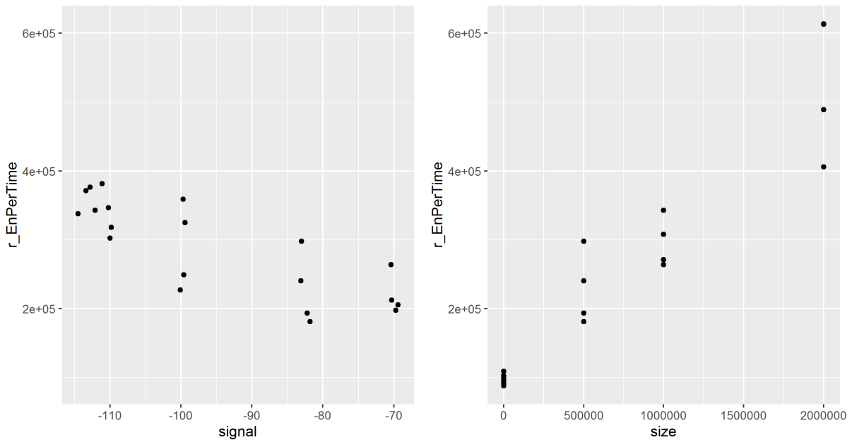
Figure 5.12: Energy per time [mJ/s] while receiving (left: size = 0.5MB ; right: -90 < signal \leq -80 )
