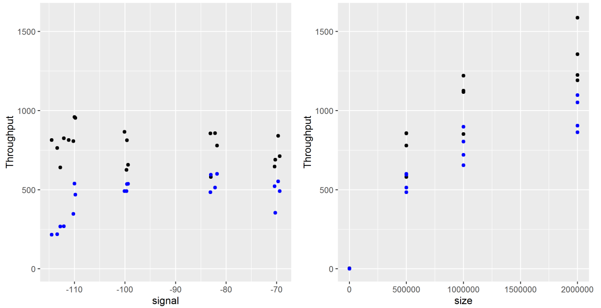
Figure 5.14: Throughput [kB/s]
