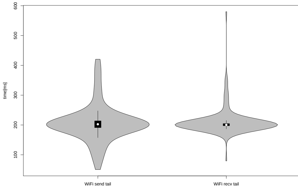
Figure 6.5: WiFi tail time violin plot
