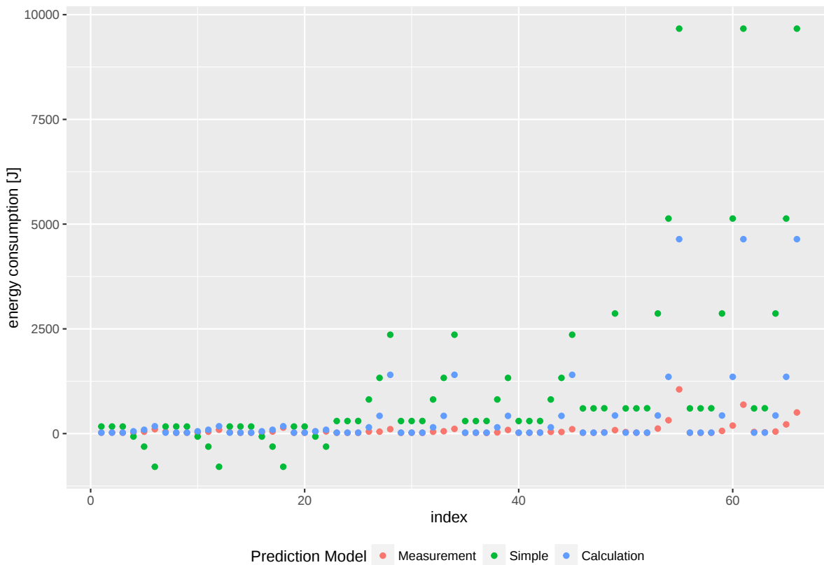
Figure 8.4: Measurement and prediction values for WiFi
