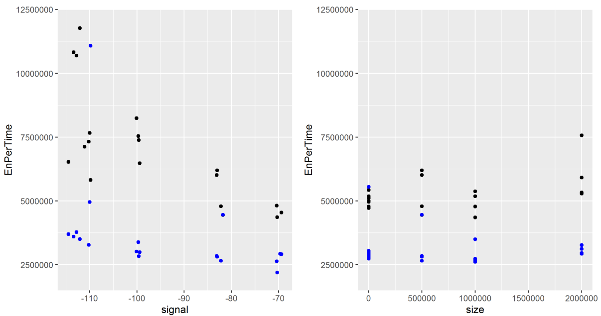
Figure 5.13: Energy per time [mJ/s] during tail time (left: size = 0.5MB ; right: -90 < signal \leq -80 ; black: receive; blue: send)
