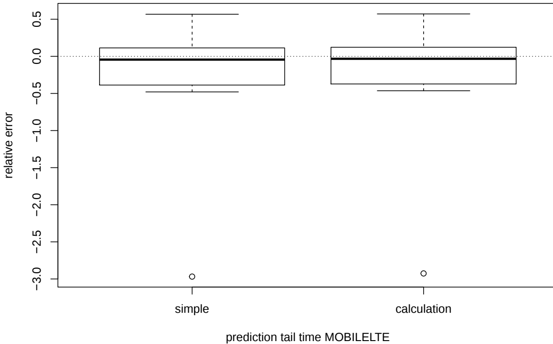
Figure 8.8: Relative error of prediction models for LTE send tail time
