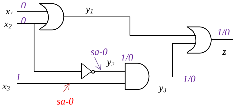
Figure 2.2: Combinational circuit
