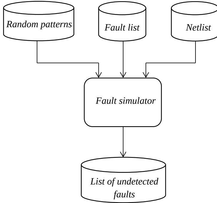
Figure 4.1: Fault simulation
