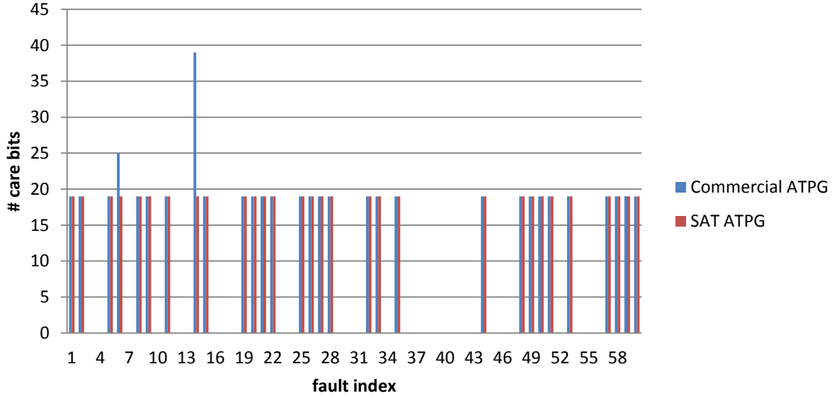
Figure 4.7: Commercial vs. SAT-based ATPG for p100k
