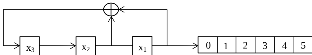
Figure 2.16: LFSR and scan chain
