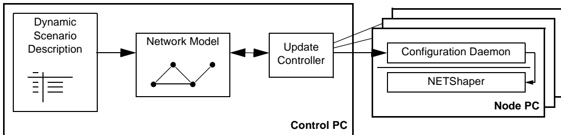
Figure 6: Emulation of a Dynamic Network Scenario.
