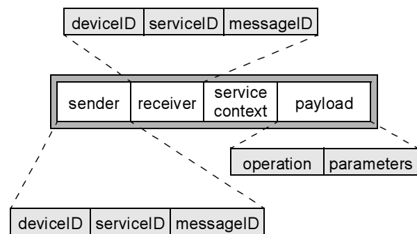
Figure 3: Invocation object structure.
