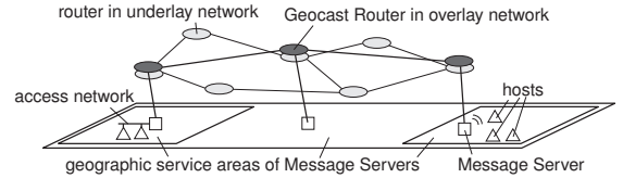
Fig. 1. System model
