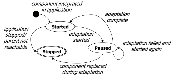
Fig. 3. Extended Component Lifecycle
