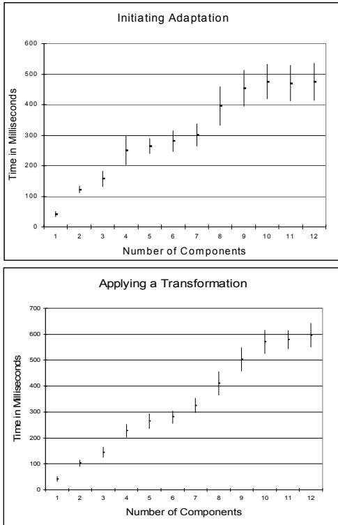
Fig. 6. Pausing (top) and Starting (bottom) a Configuration with Varying Number of Components
