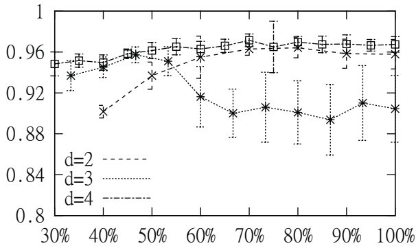
Figure 11: Maximum system load that can be served w.r.t. index depth for a small hot spot.
